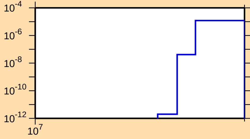
\sigma vs. E for ^{41}\text{Ca}(n,\text{pd})
