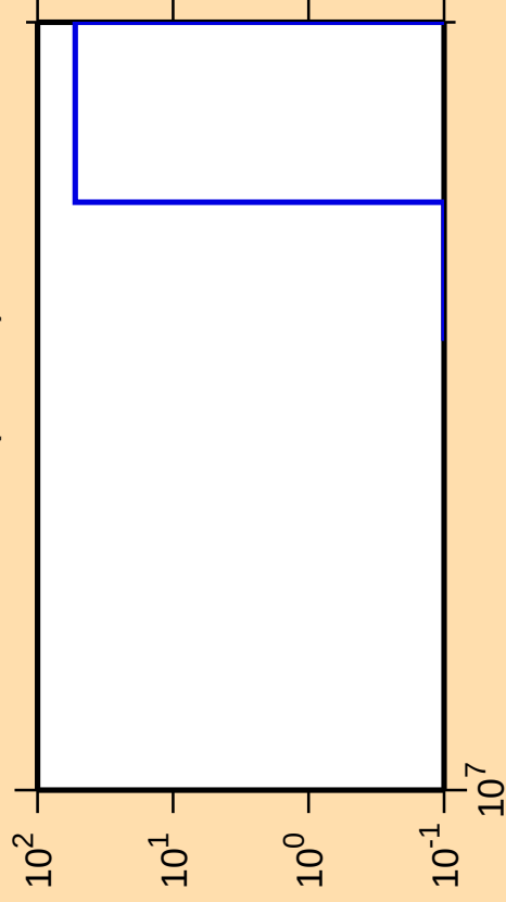
\Delta\sigma/\sigma vs. E for ^{41}\text{Ca}(\text{mt } 45)
