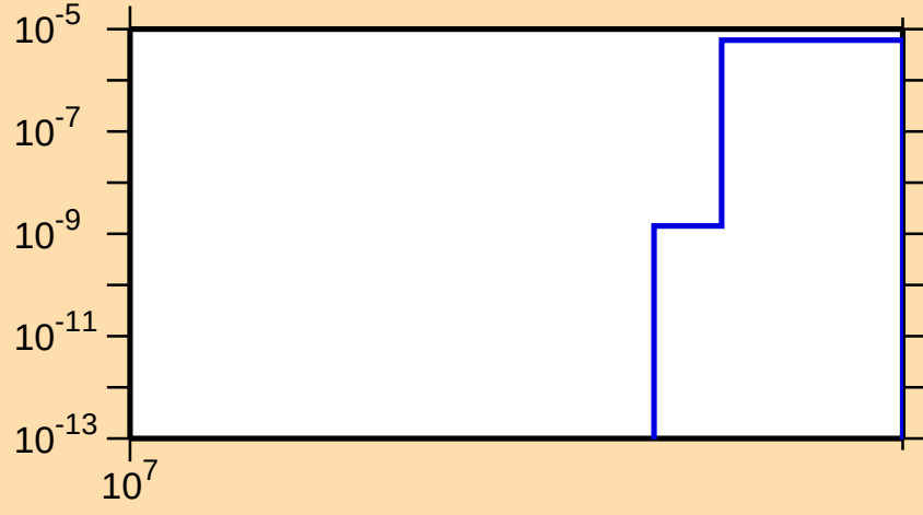
\sigma vs. E for ^{41}\text{Ca}(n,\text{pt})
