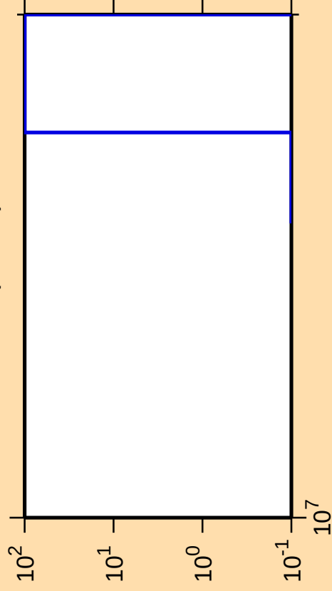
\Delta\sigma/\sigma vs. E for ^{41}\text{Ca}(\text{mt } 34)
