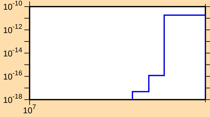
\sigma vs. E for ^{41}\text{Ca}(\text{mt } 45)
