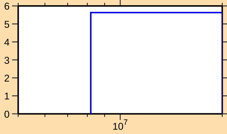
\Delta\sigma/\sigma vs. E for ^{41}\text{Ca}(n,\text{tot.})
