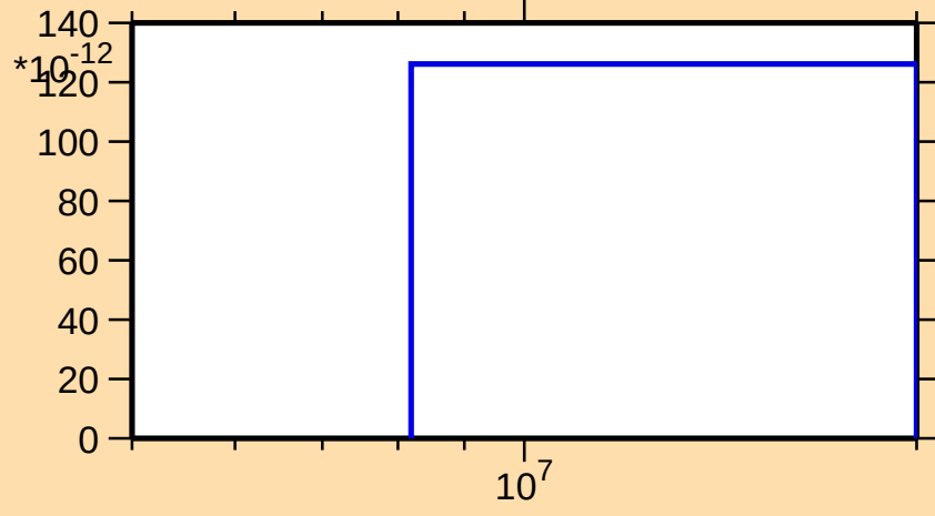
\sigma vs. E for ^{41}\text{Ca}(\text{mt } 34)
