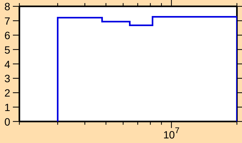
\Delta\sigma/\sigma vs. E for ^{41}\text{Ca}(n,n\text{onel.})
