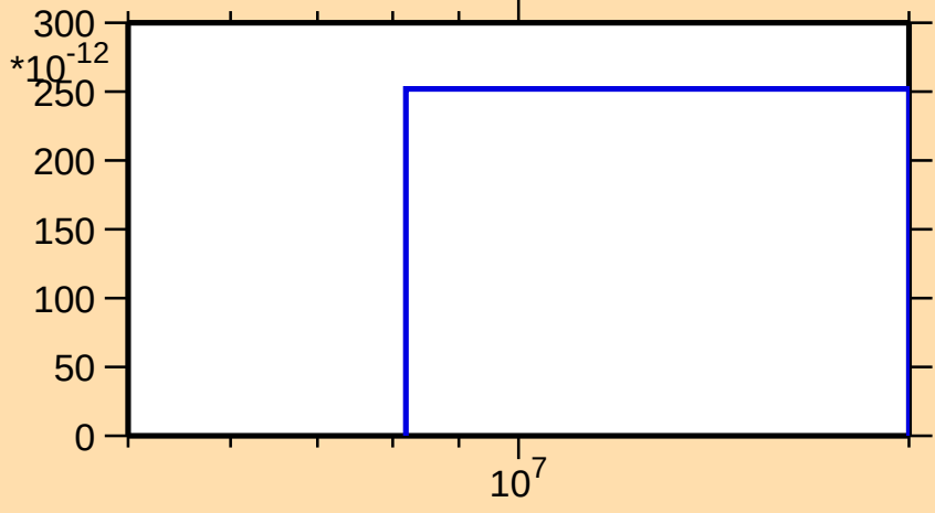
\sigma vs. E for ^{41}\text{Ca}(n,2n\alpha)
