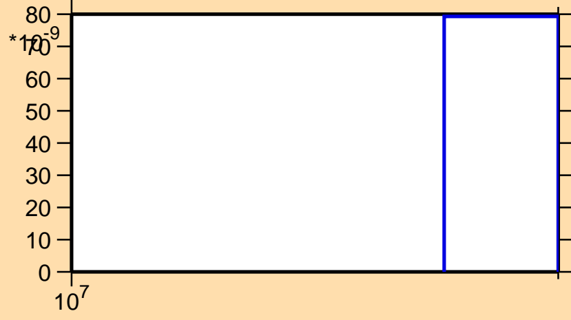
\sigma vs. E for ^{45}\text{Ca}(n,\text{nd})
