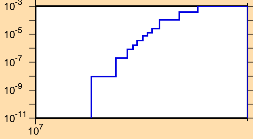
\sigma vs. E for ^{45}\text{Ca}(n,t)
