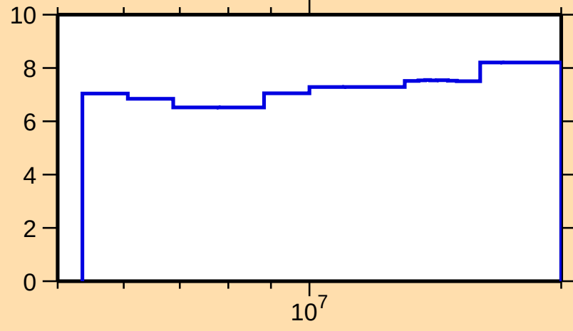
\Delta\sigma/\sigma vs. E for ^{46}\text{Ca}(n,n\text{oncl.})
