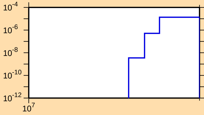
\sigma vs. E for ^{46}\text{Ca}(n,t)
