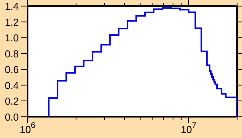
\sigma vs. E for ^{46}\text{Ca}(n,\text{inel.})
