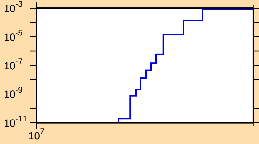
\sigma vs. E for ^{46}\text{Ca}(n,n\alpha)
