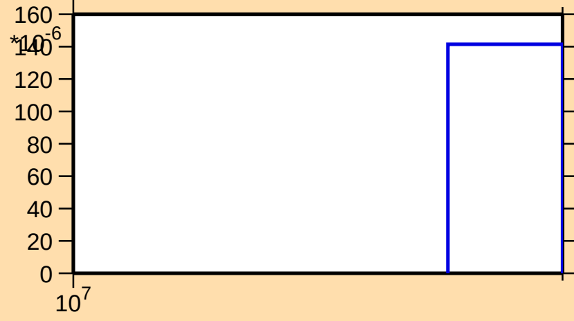
\sigma vs. E for ^{46}\text{Ca}(n,3n)
