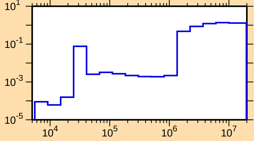
\sigma vs. E for ^{46}\text{Ca}(n,\text{nonel.})
