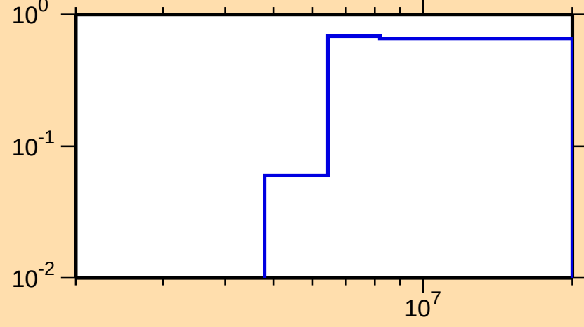
\sigma vs. E for ^{46}\text{Ca}(n,n\text{cont.})
