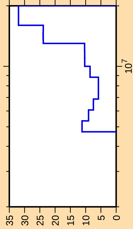
\Delta\sigma/\sigma vs. E for ^{47}\text{Ca}(n,\text{ncont.})
