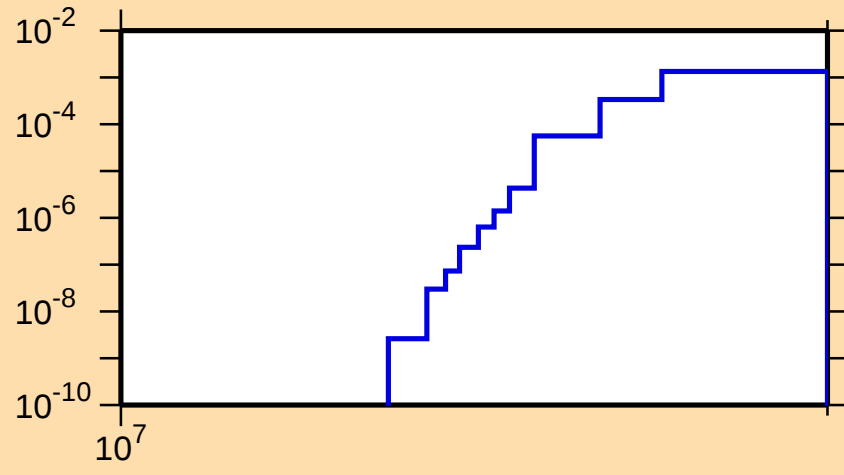
\sigma vs. E for ^{47}\text{Ca}(n,d)
