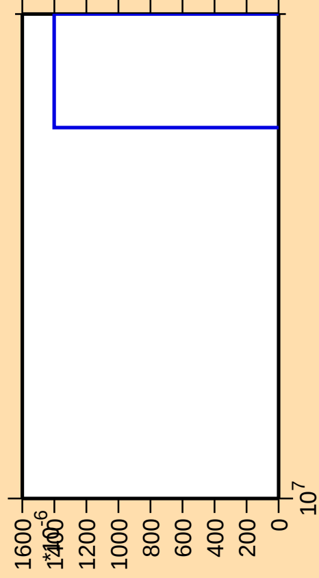
\Delta\sigma/\sigma vs. E for ^{47}\text{Ca}(n,2n\alpha)
