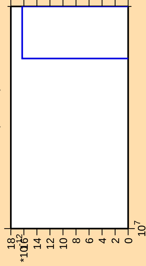
\Delta\sigma/\sigma vs. E for ^{47}\text{Ca}(n,\text{He}3)
