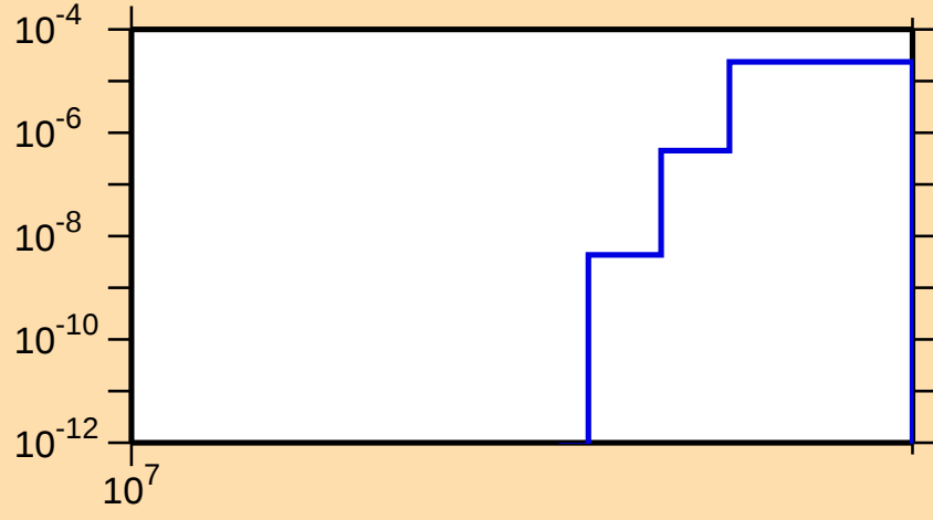
\sigma vs. E for ^{47}\text{Ca}(n,n\alpha)
