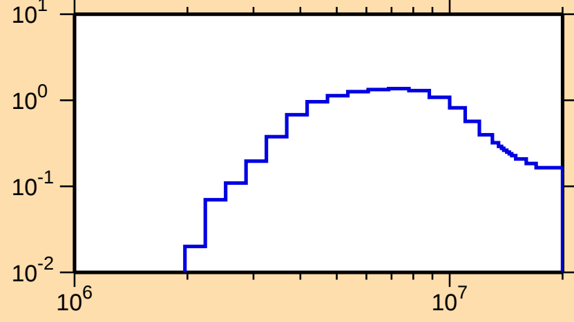
\sigma vs. E for ^{47}\text{Ca}(n,\text{inel.})
