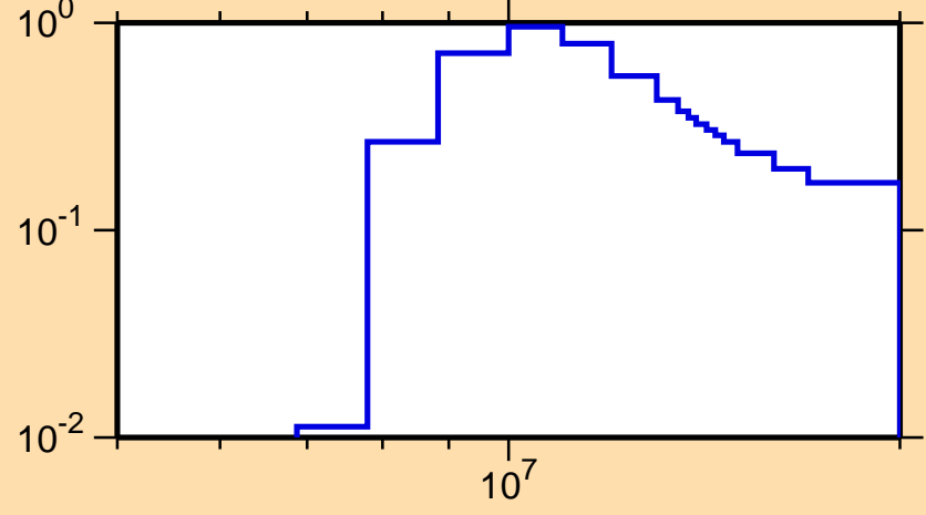
\sigma vs. E for ^{48}\text{Ca}(n,n\text{cont.})
