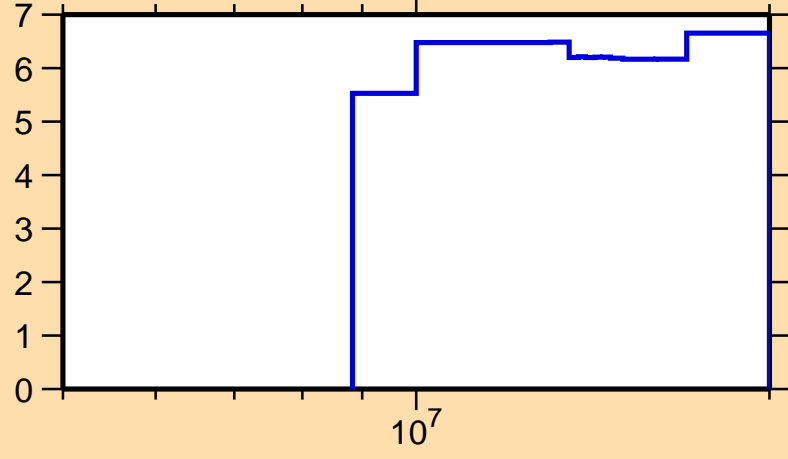
\Delta\sigma/\sigma vs. E for ^{48}\text{Ca}(n,\text{nonel.})
