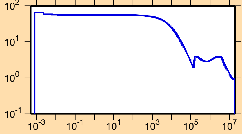
\sigma vs. E for ^{48}\text{Ca}(n,\text{el.})
