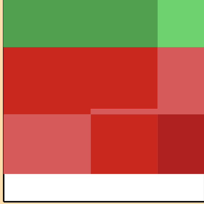
\Delta\sigma/\sigma vs. E for ^{48}\text{Ca}(n,\text{inel.})
