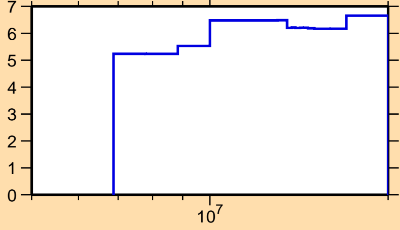
\Delta\sigma/\sigma vs. E for ^{48}\text{Ca}(n,n\text{onel.})
