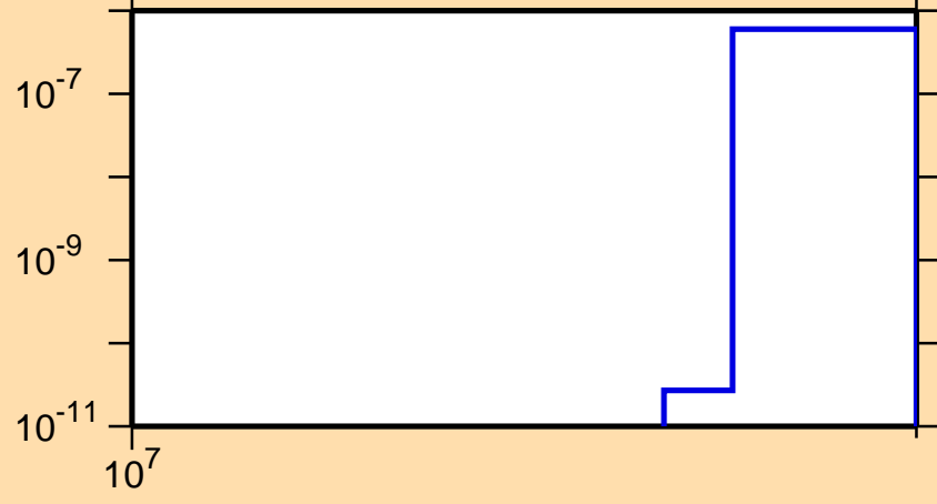
\sigma vs. E for ^{48}\text{Ca}(n,t)
