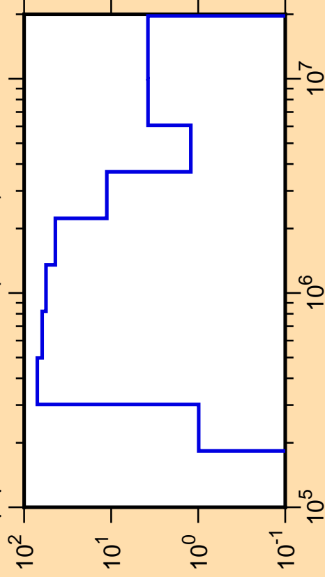
\Delta\mu/\mu vs. E for ^{48}\text{Ca}(\text{mt251})
