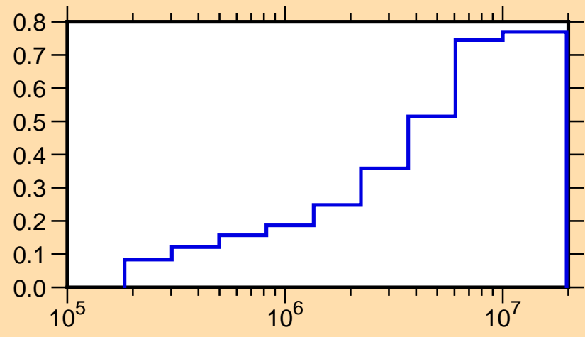
\mu vs. E for ^{48}\text{Ca}(\text{mt251})
