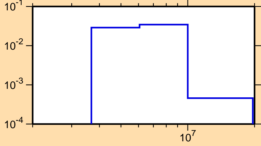
\sigma vs. E for ^{48}\text{Ca}(n,n_2)
