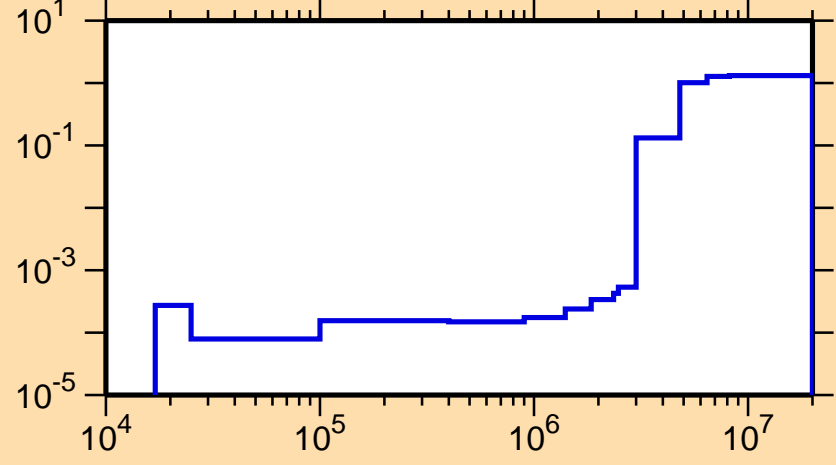
\sigma vs. E for ^{48}\text{Ca}(n,\text{nonel.})
