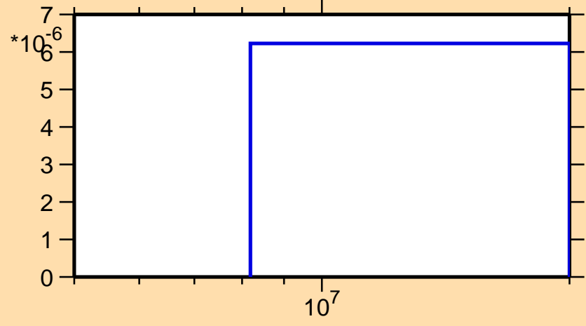
\sigma vs. E for ^{48}\text{Ca}(n,3n)
