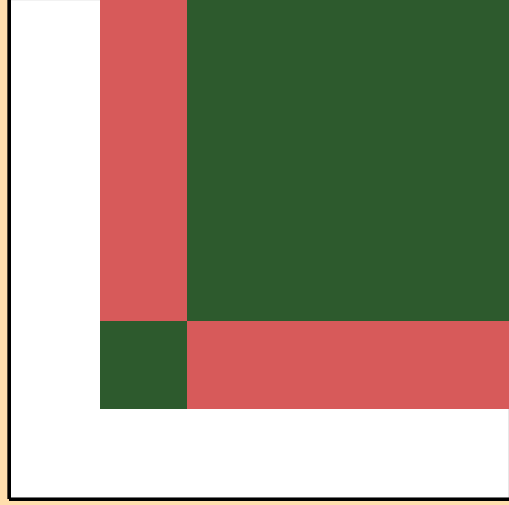
\sigma vs. E for ^{48}\text{Ca}(n,n\text{cont.})
