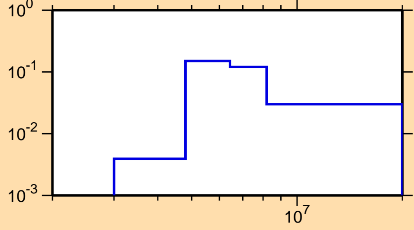
\sigma vs. E for ^{48}\text{Ca}(n,n_4)
