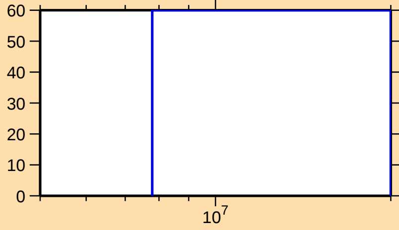
\Delta\sigma/\sigma vs. E for ^{50}\text{Ca}(n,\text{ncont.})
