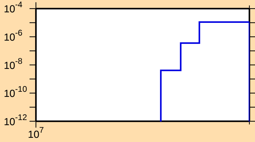
\sigma vs. E for ^{50}\text{Ca}(n,t)
