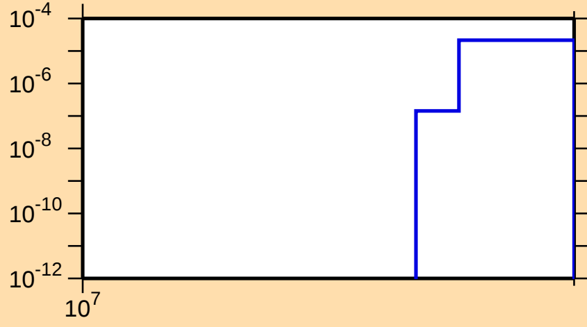
\sigma vs. E for ^{50}\text{Ca}(n,d)
