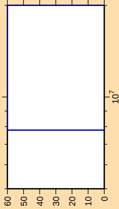
\Delta\sigma/\sigma vs. E for ^{50}\text{Ca}(n,\text{ncont.})
