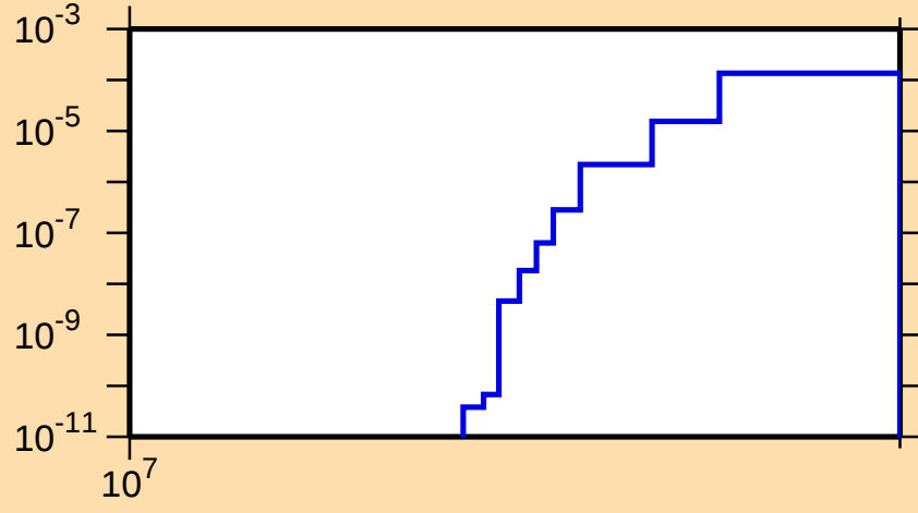
\sigma vs. E for ^{50}\text{Ca}(n,p)
