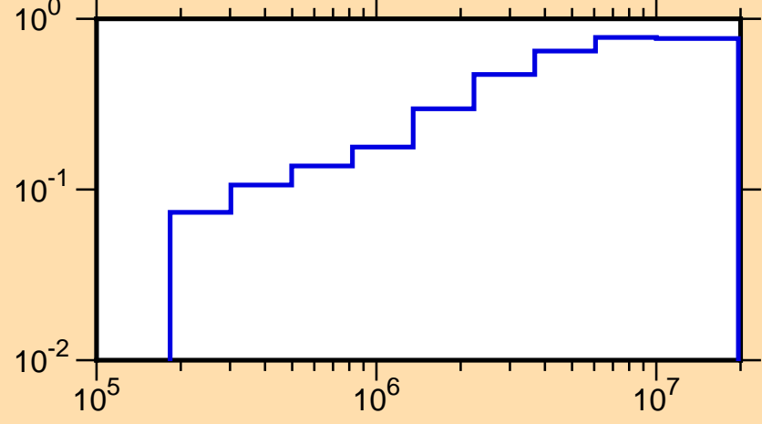
\mu vs. E for ^{50}\text{Ca}(\text{mt251})
