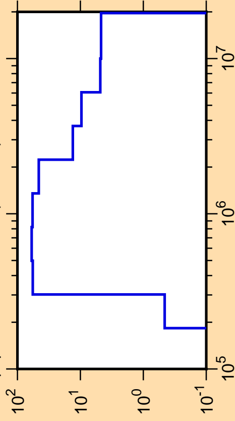
\Delta\mu/\mu vs. E for ^{50}\text{Ca}(\text{mt251})
