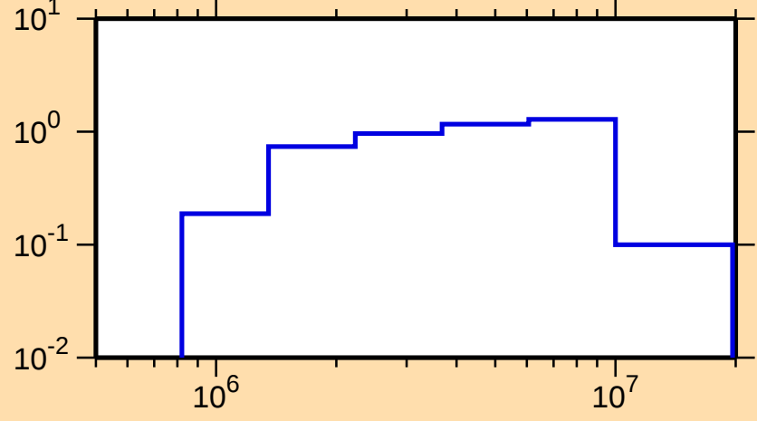
\sigma vs. E for ^{50}\text{Ca}(n,\text{inel.})
