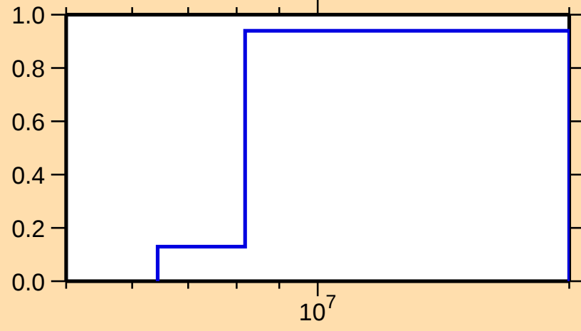
\sigma vs. E for ^{50}\text{Ca}(n,2n)
