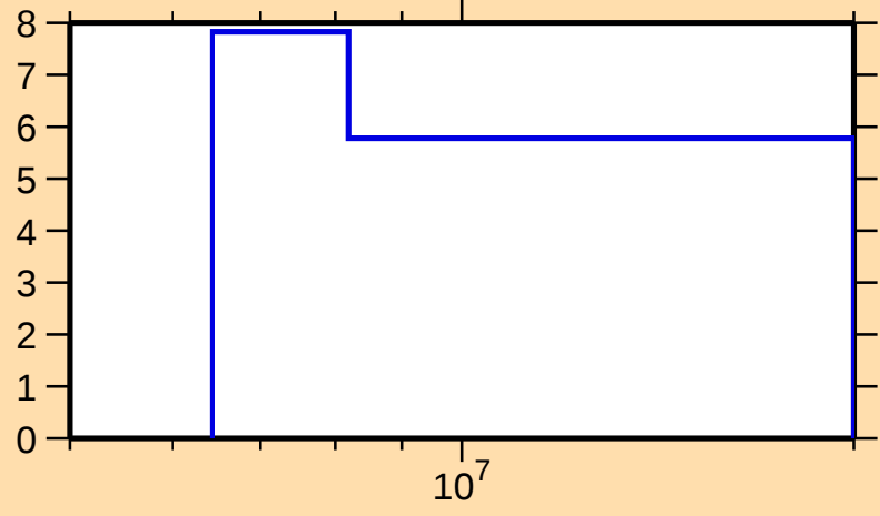
\Delta\sigma/\sigma vs. E for ^{50}\text{Ca}(n,n\text{onel.})
