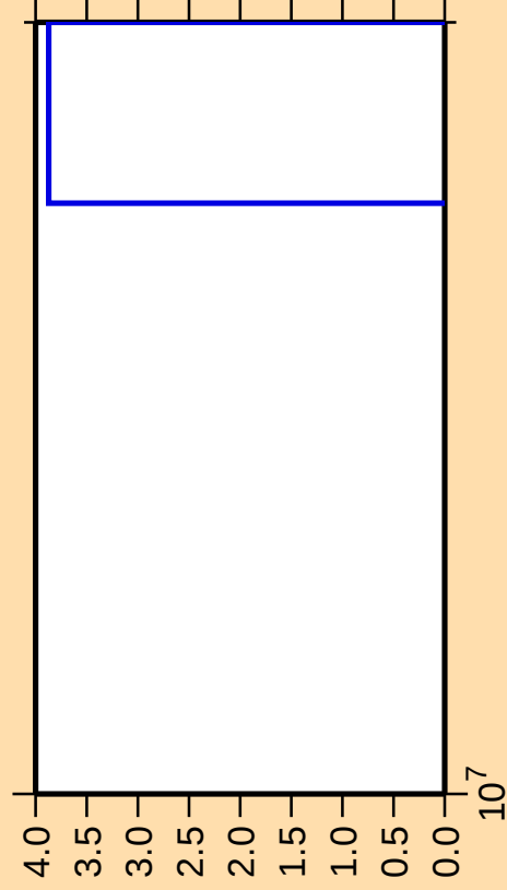
\Delta\sigma/\sigma vs. E for ^{98}\text{Cd}(n,2np)
