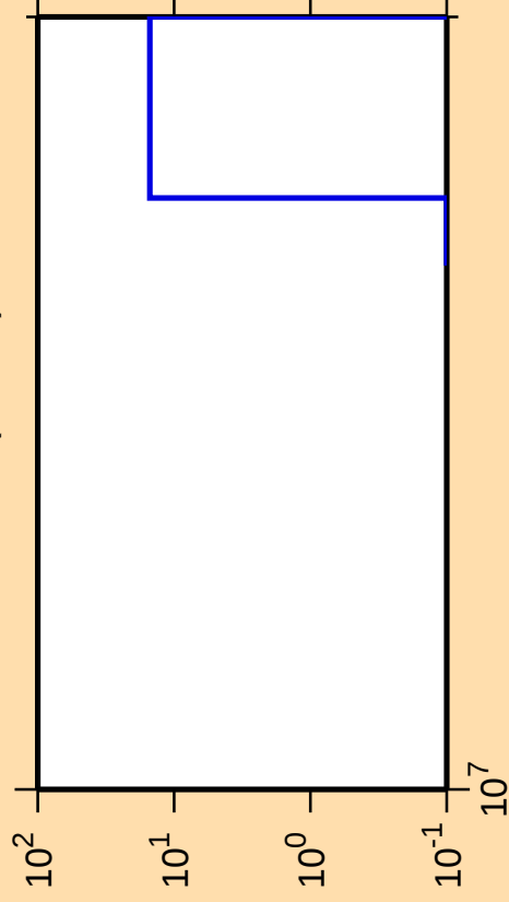
\Delta\sigma/\sigma vs. E for ^{98}\text{Cd}(\text{mt } 34)
