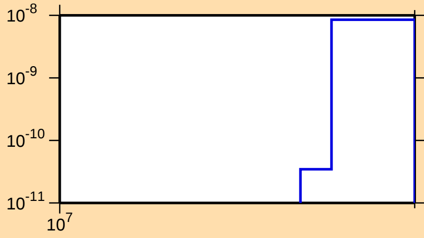
\sigma vs. E for ^{98}\text{Cd}(\text{mt } 45)
