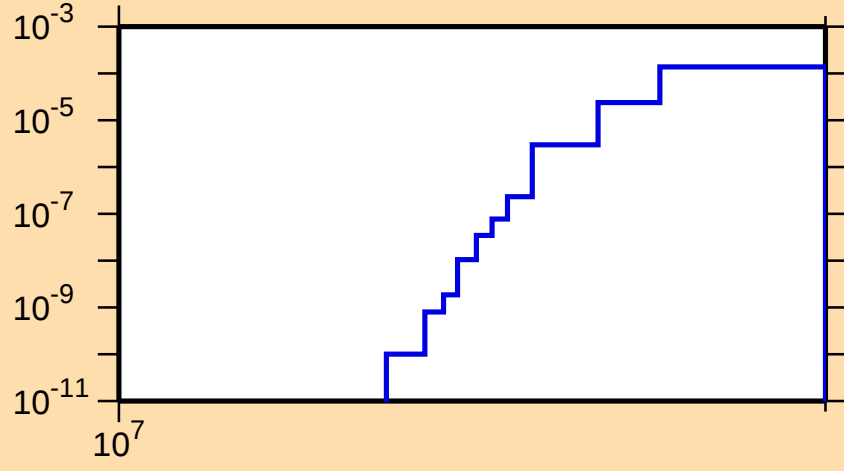
\sigma vs. E for ^{98}\text{Cd}(n,t)
