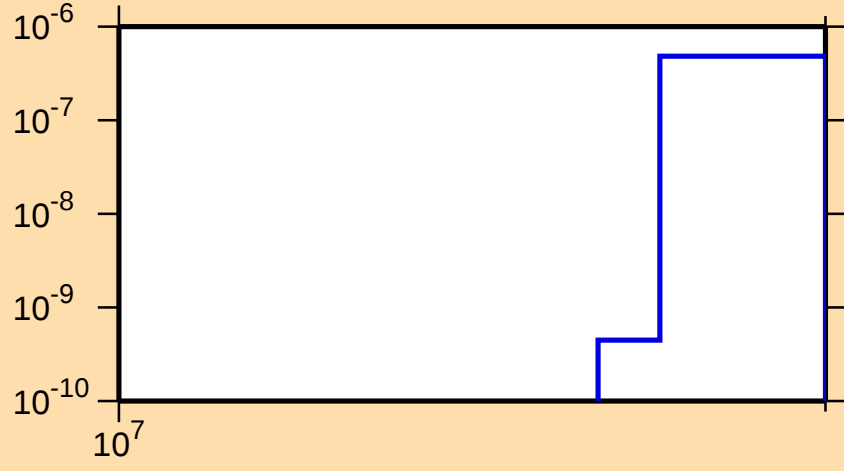
\sigma vs. E for ^{98}\text{Cd}(n,\text{pt})
