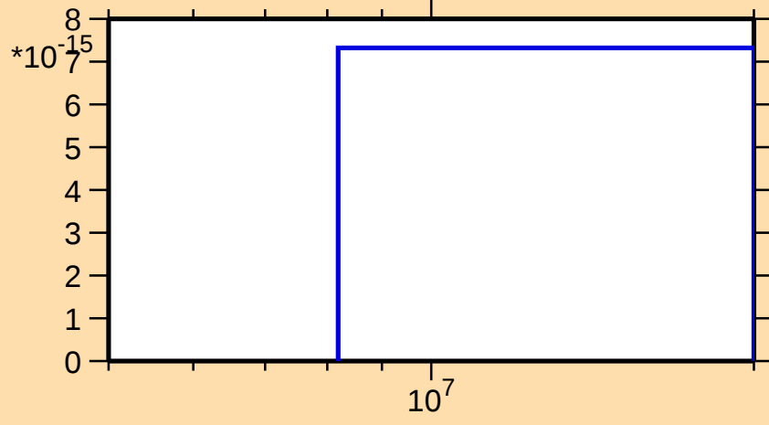
\sigma vs. E for ^{98}\text{Cd}(n,2np)
