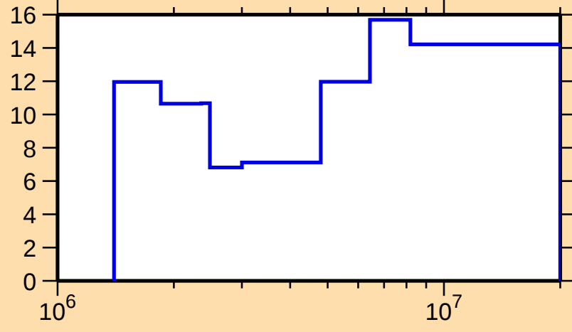
\Delta\sigma/\sigma vs. E for ^{98}\text{Cd}(\text{n,nonel.})
