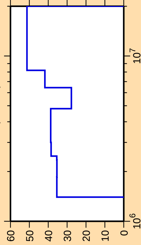
\Delta\sigma/\sigma vs. E for ^{98}\text{Cd}(\text{n,inel.})
