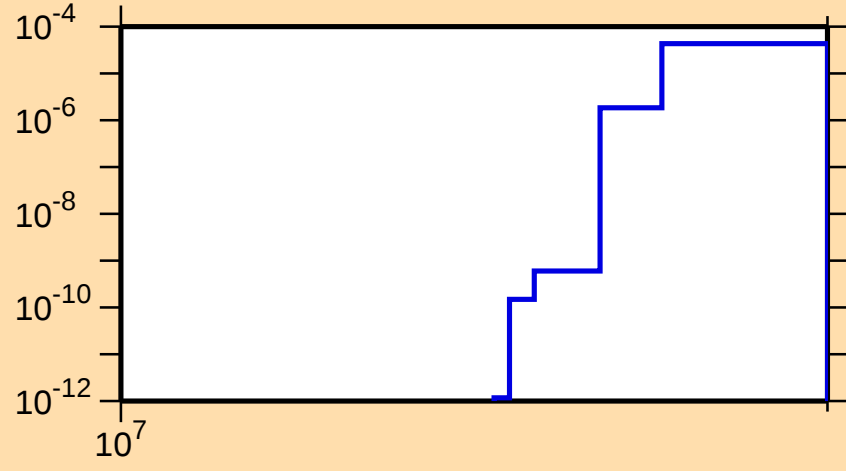
\sigma vs. E for ^{99}\text{Cd}(n,2np)
