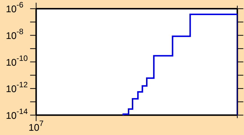
\sigma vs. E for ^{99}\text{Cd}(\text{mt } 45)
