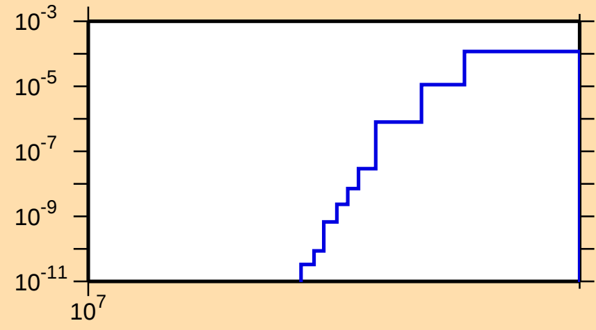
\sigma vs. E for ^{99}\text{Cd}(n,\text{pt})
