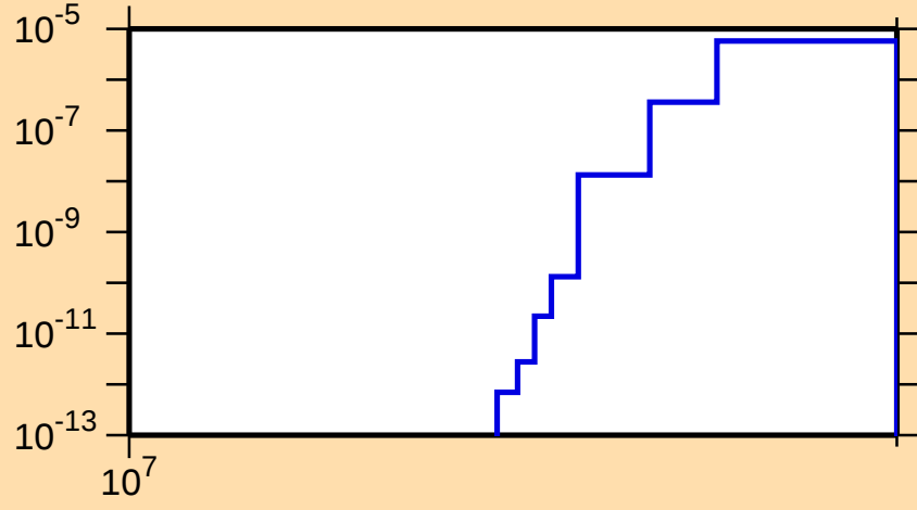
\sigma vs. E for ^{99}\text{Cd}(n,\text{nd})
