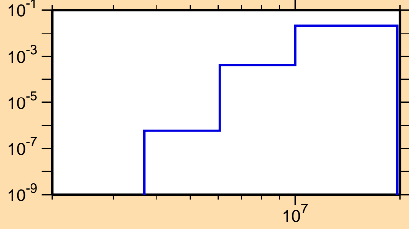
\sigma vs. E for ^{99}\text{Cd}(n,d)
