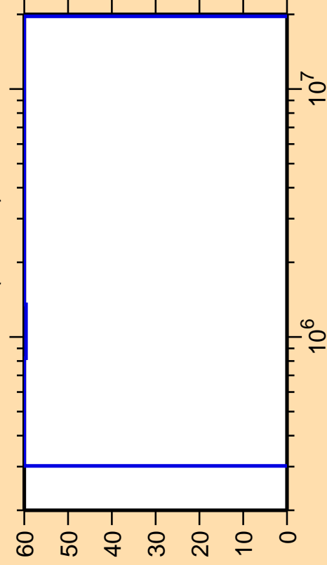
\Delta\sigma/\sigma vs. E for ^{99}\text{Cd}(n,\text{inel.})
