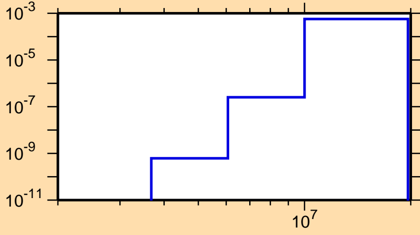
\sigma vs. E for ^{99}\text{Cd}(n,\text{He3})
