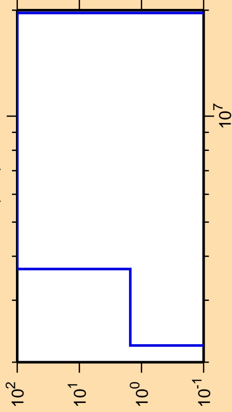
\Delta\sigma/\sigma vs. E for ^{99}\text{Cd}(n,d)
