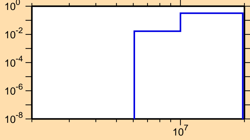
\sigma vs. E for ^{99}\text{Cd}(n,np)
