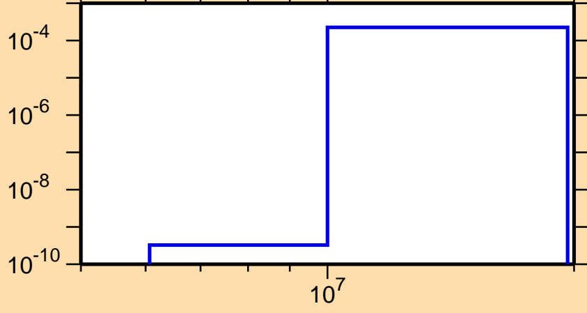
\sigma vs. E for ^{99}\text{Cd}(n,t)
