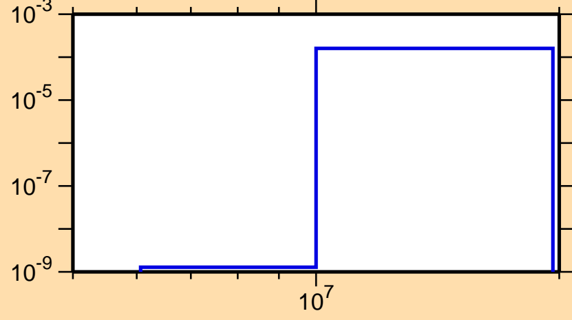
\sigma vs. E for ^{99}\text{Cd}(n,\alpha)
