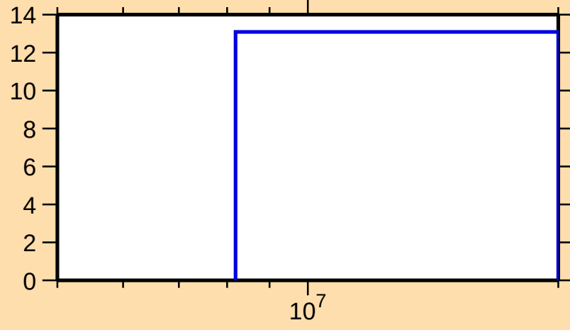
\Delta\sigma/\sigma vs. E for ^{99}\text{Cd}(n,\text{tot.})
