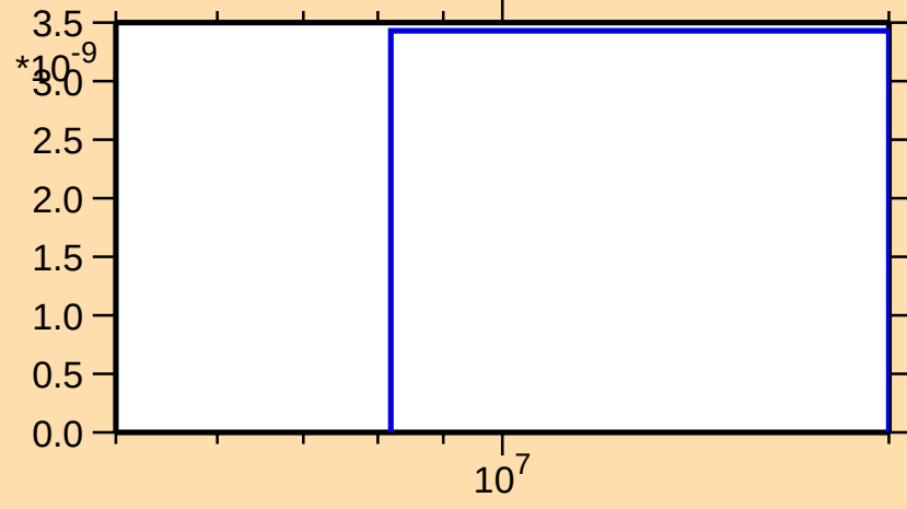
\sigma vs. E for ^{99}\text{Cd}(\text{mt } 45)
