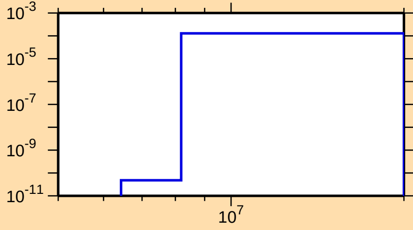
\sigma vs. E for ^{99}\text{Cd}(n,n\alpha)
