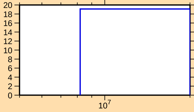
\Delta\sigma/\sigma vs. E for ^{99}\text{Cd}(n,\text{nonel.})
