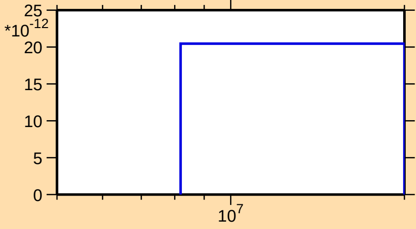
\sigma vs. E for ^{99}\text{Cd}(\text{mt117})
