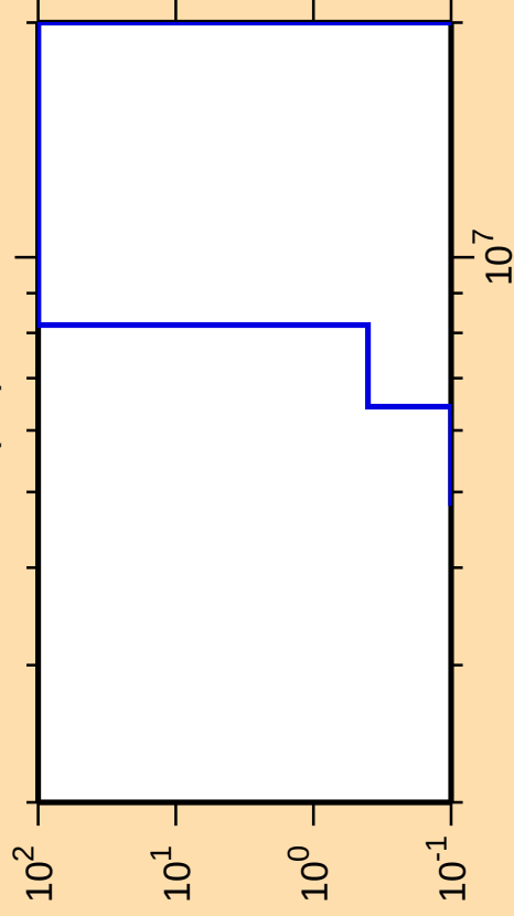
\Delta\sigma/\sigma vs. E for ^{99}\text{Cd}(n,t)
