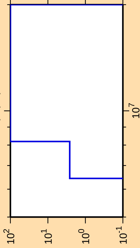
\Delta\sigma/\sigma vs. E for ^{99}\text{Cd}(n,\text{pd})
