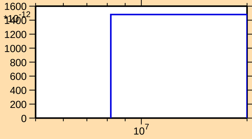
\sigma vs. E for ^{99}\text{Cd}(\text{mt } 34)
