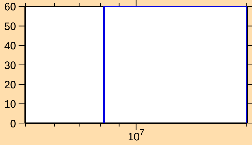
\Delta\sigma/\sigma vs. E for ^{99}\text{Cd}(n,\text{inel.})
