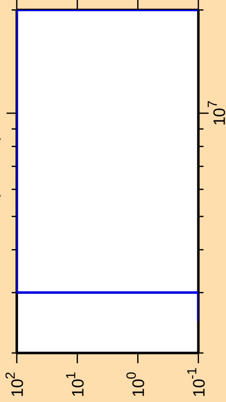
\Delta\sigma/\sigma vs. E for ^{99}\text{Cd}(n,\text{He3})
