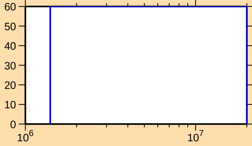
\Delta\sigma/\sigma vs. E for ^{99}\text{Cd}(n,n_1)
