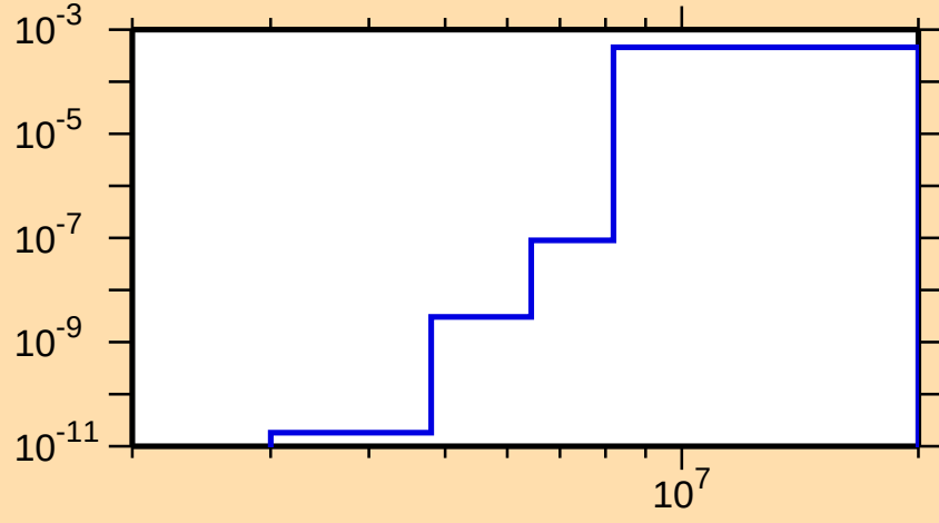
\sigma vs. E for ^{99}\text{Cd}(n,\text{He3})
