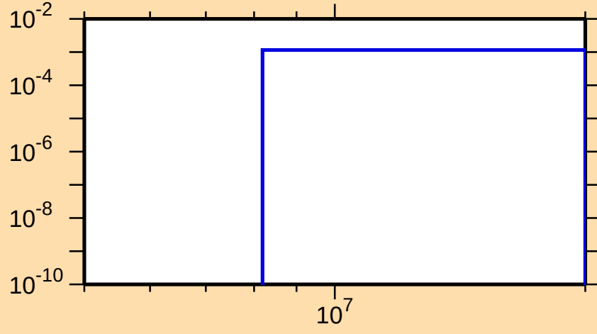
\sigma vs. E for ^{99}\text{Cd}(n,\text{pd})
