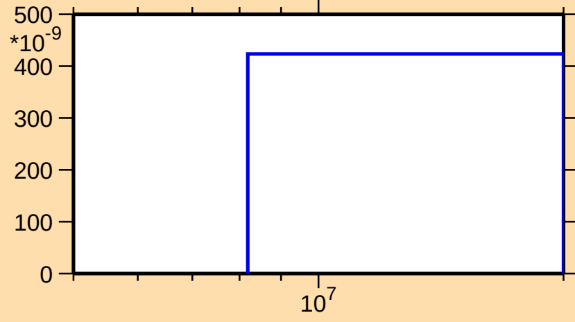
\sigma vs. E for ^{99}\text{Cd}(n,2np)
