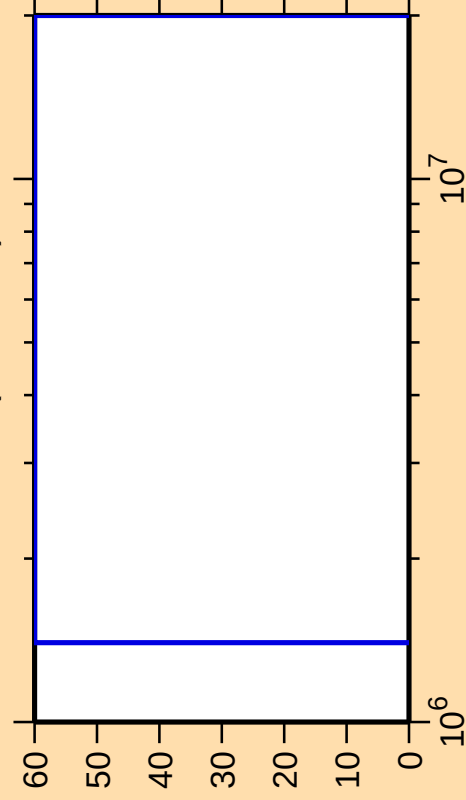
\Delta\sigma/\sigma vs. E for ^{99}\text{Cd}(n,\text{ncont.})
