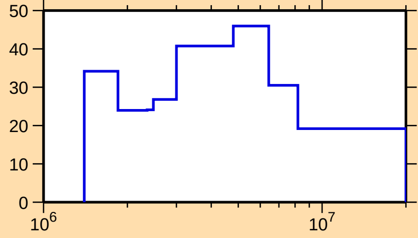
\Delta\sigma/\sigma vs. E for ^{99}\text{Cd}(n,\text{el.})
