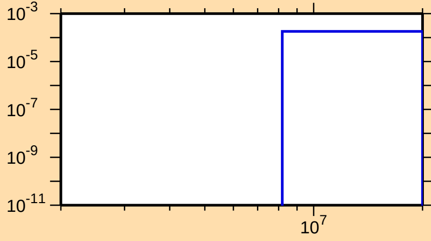
\sigma vs. E for ^{99}\text{Cd}(n,t)
