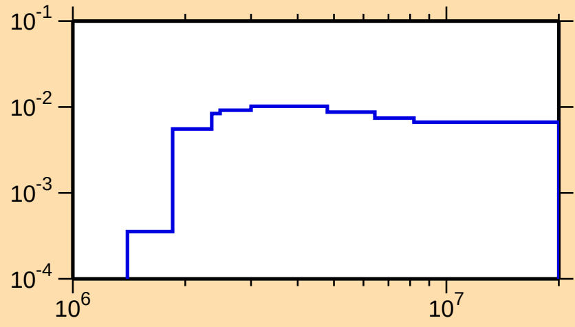
\sigma vs. E for ^{99}\text{Cd}(n,n\text{cont.})
