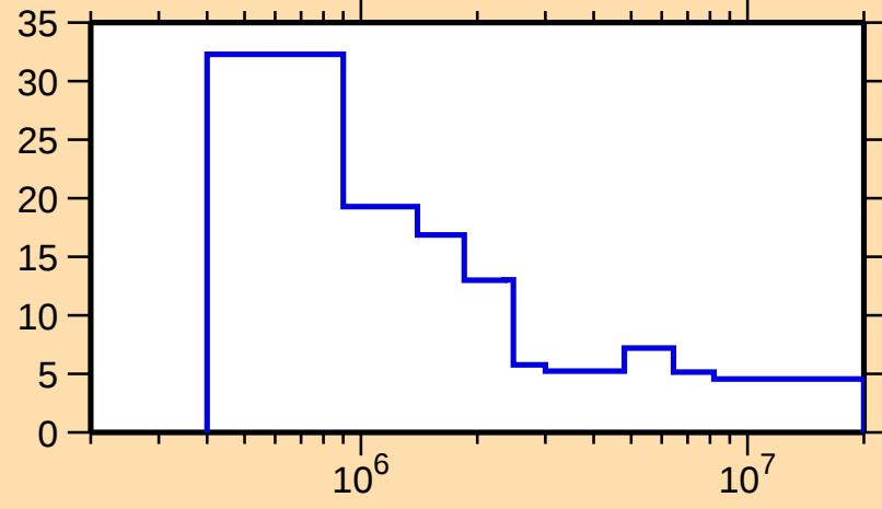
\Delta\sigma/\sigma vs. E for ^{104}\text{Cd}(\text{n,nonel.})
