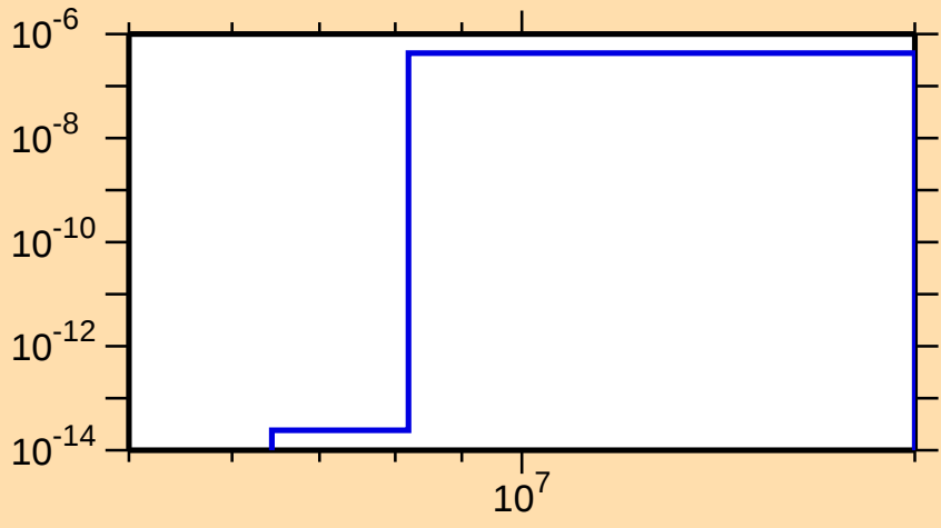
\sigma vs. E for ^{104}\text{Cd}(n,\text{He}3)
