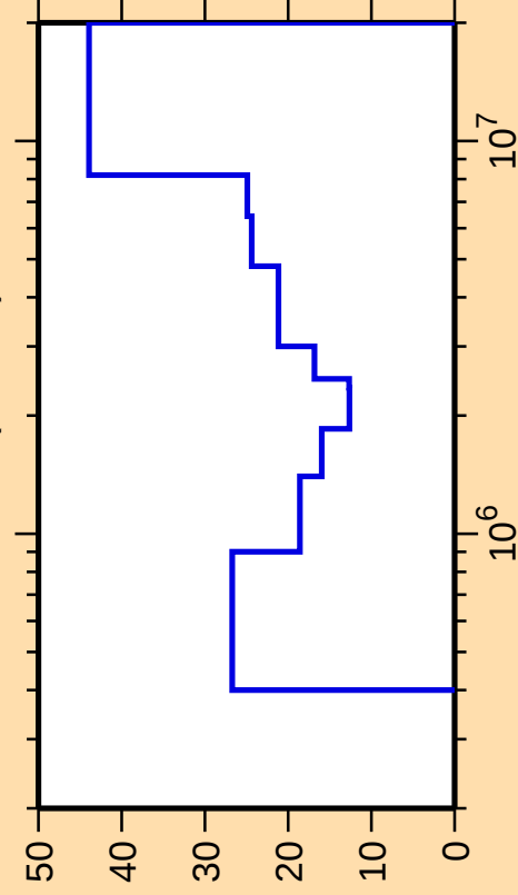
\Delta\sigma/\sigma vs. E for ^{104}\text{Cd}(\text{n,inel.})
