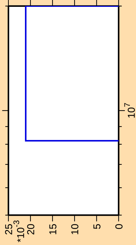
\Delta\sigma/\sigma vs. E for ^{104}\text{Cd}(n,\text{nt})
