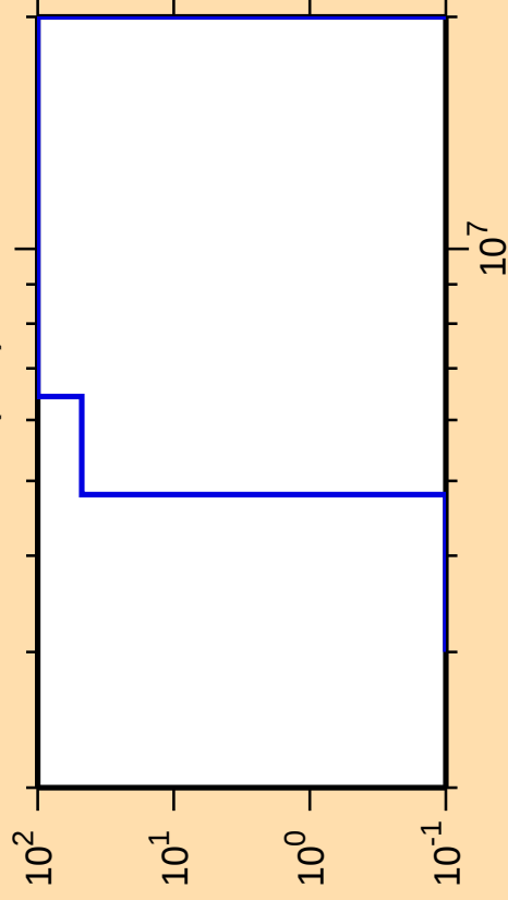
\Delta\sigma/\sigma vs. E for ^{104}\text{Cd}(n,d)
