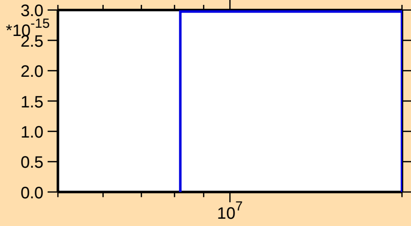
\sigma vs. E for ^{104}\text{Cd}(n,\text{nt})
