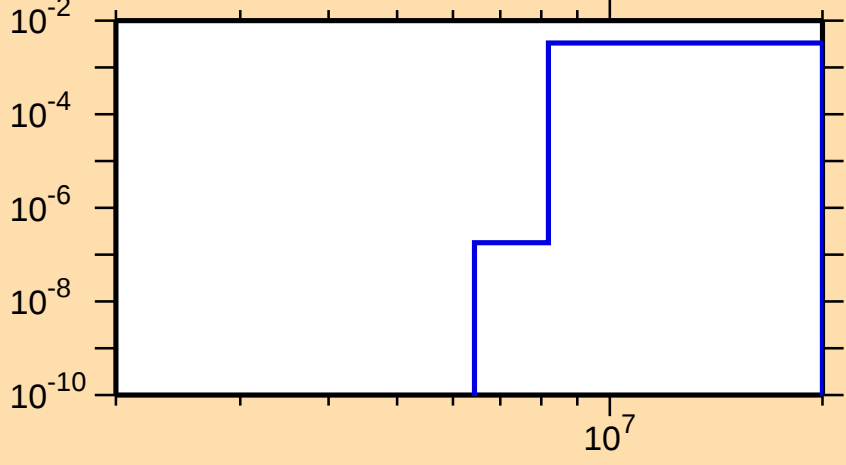
\sigma vs. E for ^{104}\text{Cd}(n,d)
