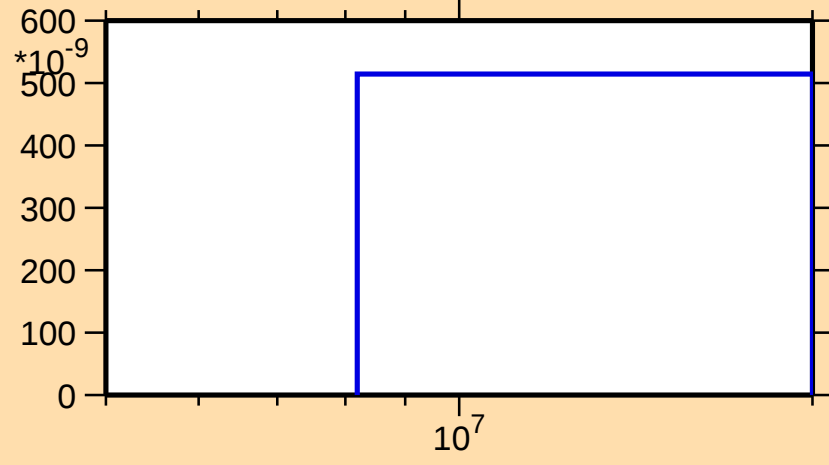
\sigma vs. E for ^{104}\text{Cd}(n,\text{pd})
