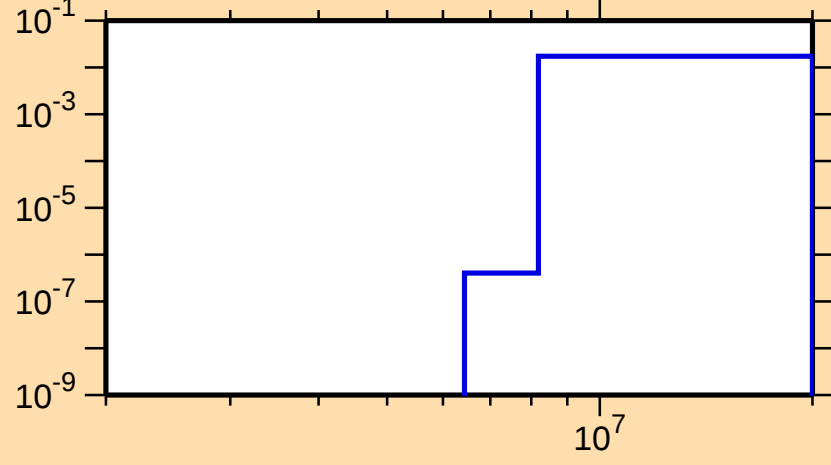
\sigma vs. E for ^{106}\text{Cd}(n,\alpha)
