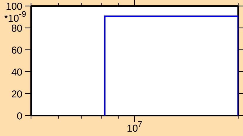
\sigma vs. E for ^{106}\text{Cd}(n,\text{He}3)
