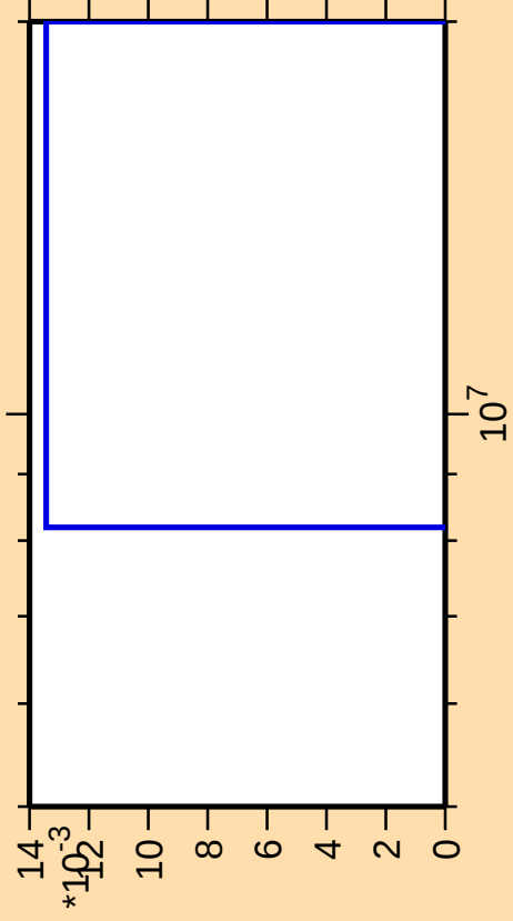
\Delta\sigma/\sigma vs. E for ^{106}\text{Cd}(n,\text{nt})
