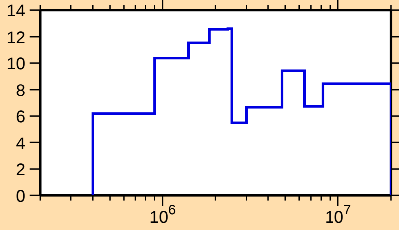
\Delta\sigma/\sigma vs. E for ^{106}\text{Cd}(\text{n,el.})
