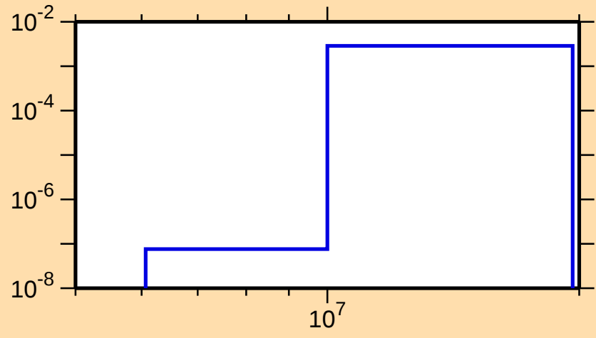
\sigma vs. E for ^{107}\text{Cd}(n,d)
