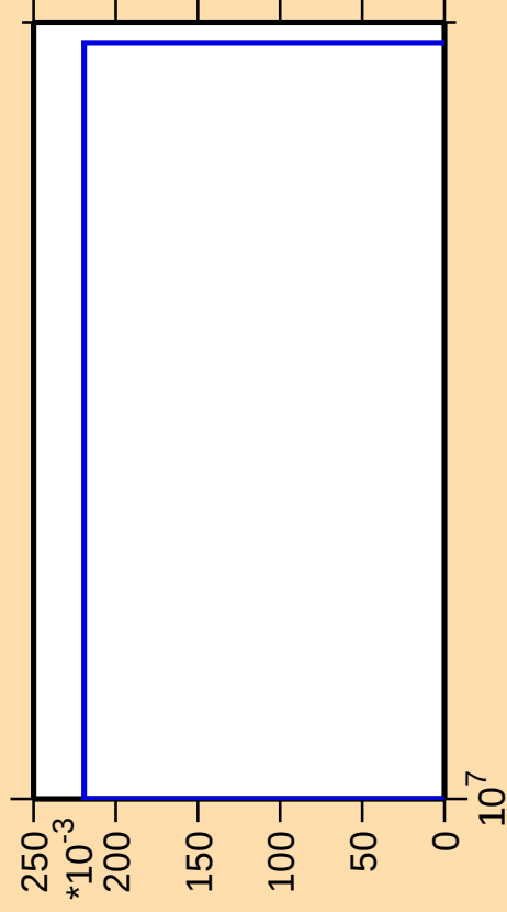
\Delta\sigma/\sigma vs. E for ^{107}\text{Cd}(\text{mt } 34)
