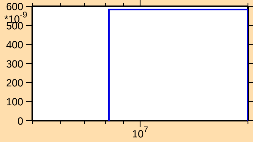
\sigma vs. E for ^{107}\text{Cd}(n,2np)
