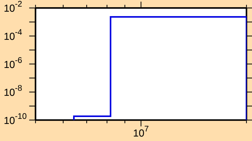
\sigma vs. E for ^{107}\text{Cd}(n,d)
