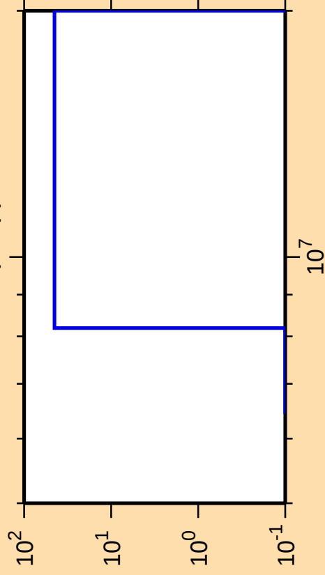
\Delta\sigma/\sigma vs. E for ^{107}\text{Cd}(n,np)
