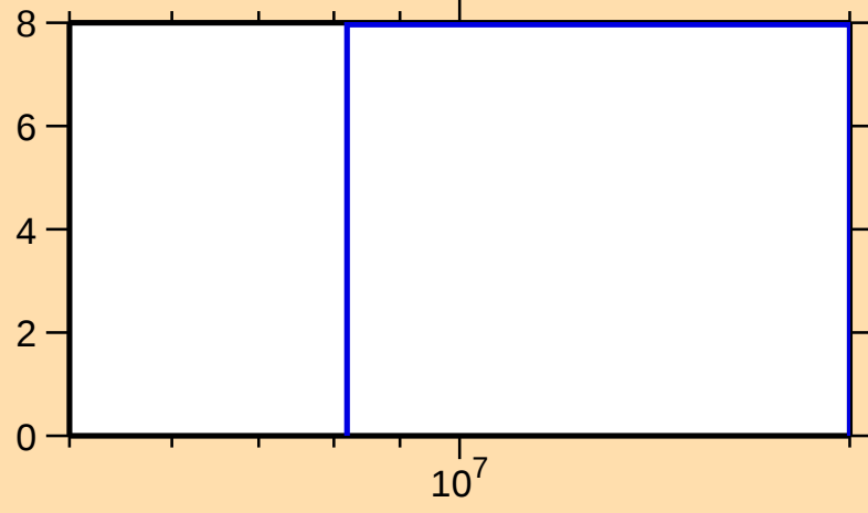
\Delta\sigma/\sigma vs. E for ^{108}\text{Cd}(n,\text{el.})
