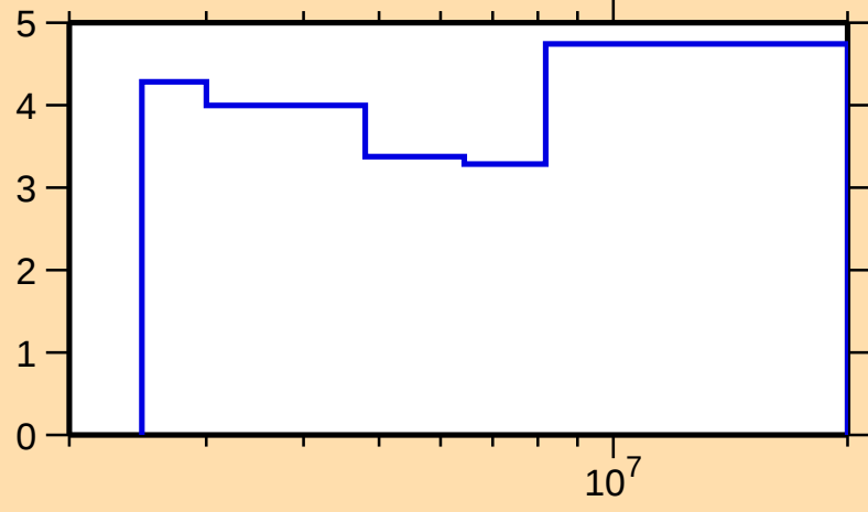
\Delta\sigma/\sigma vs. E for ^{108}\text{Cd}(\text{n},\text{tot.})
