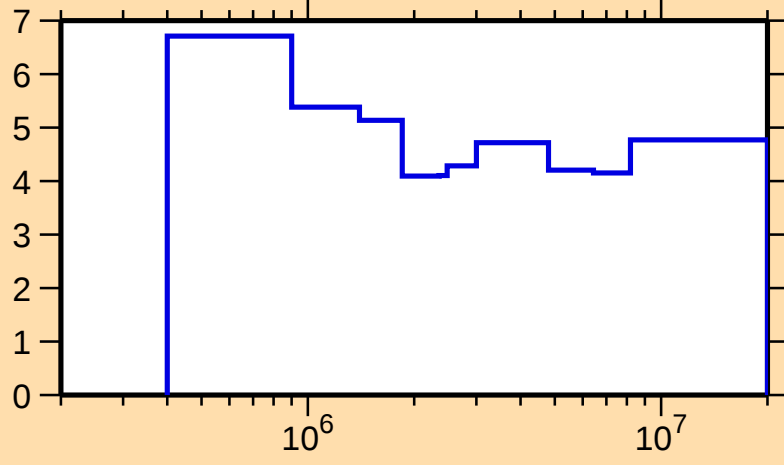
\Delta\sigma/\sigma vs. E for ^{108}\text{Cd}(\text{n,nonel.})
