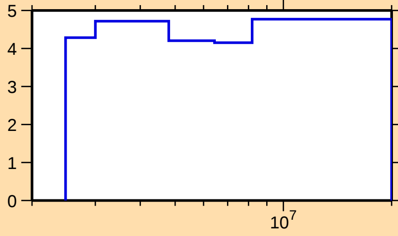
\Delta\sigma/\sigma vs. E for ^{108}\text{Cd}(\text{n},\text{nonel.})
