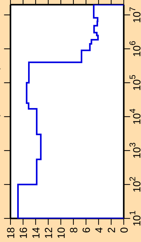
\Delta\sigma/\sigma vs. E for ^{108}\text{Cd}(n,\text{nonel.})
