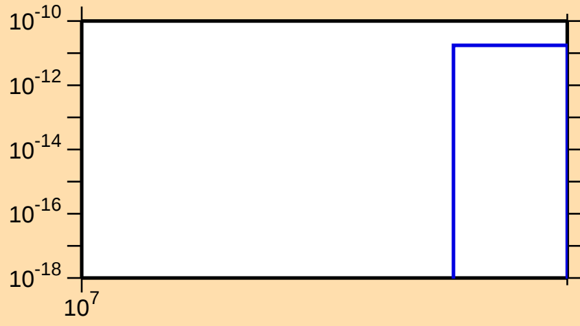
\sigma vs. E for ^{111}\text{Cd}(n,\text{nt})
