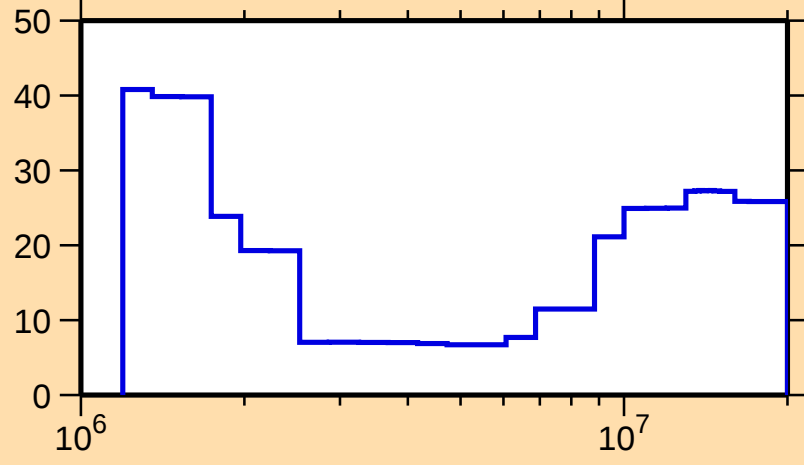
\Delta\sigma/\sigma vs. E for ^{111}\text{Cd}(n,n\text{cont.})
