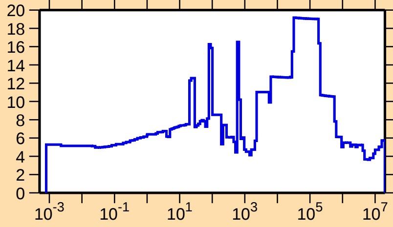
\Delta\sigma/\sigma vs. E for ^{111}\text{Cd}(n,\text{tot.})
