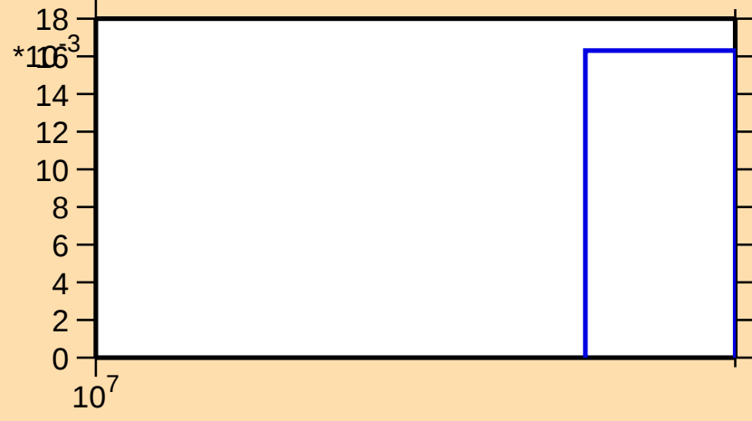
\sigma vs. E for ^{111}\text{Cd}(n,3n)
