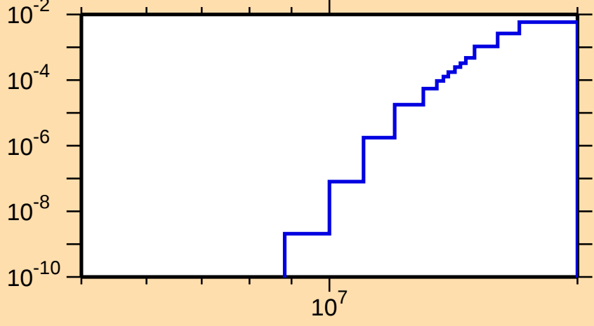
\sigma vs. E for ^{111}\text{Cd}(n,\alpha)
