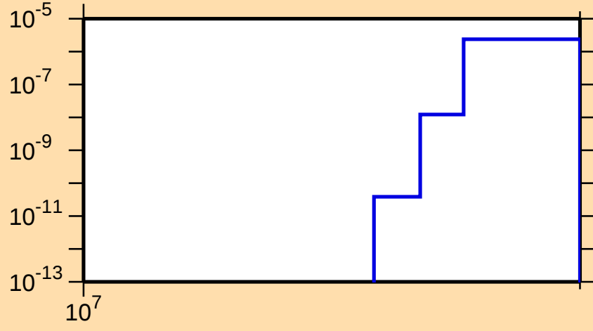
\sigma vs. E for ^{111}\text{Cd}(n,\text{nd})
