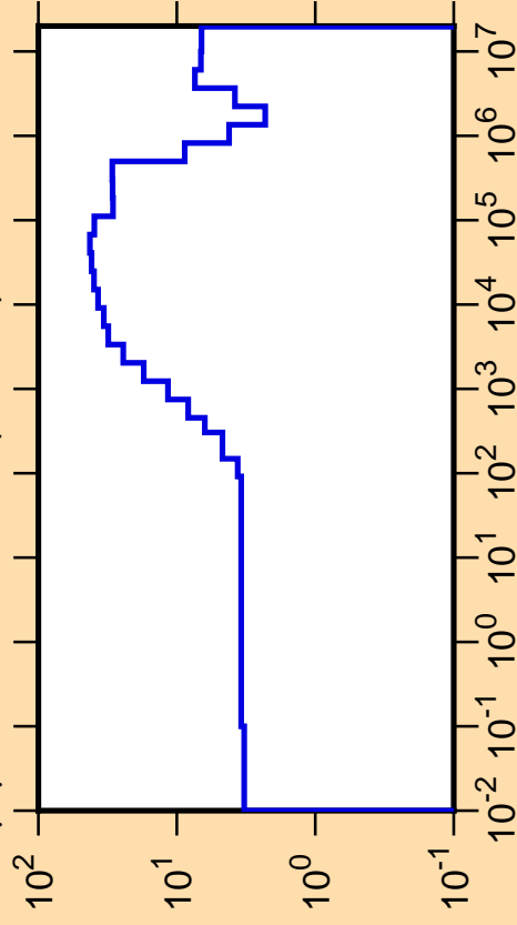
\Delta\mu/\mu vs. E for ^{111}\text{Cd}(\text{mt251})
