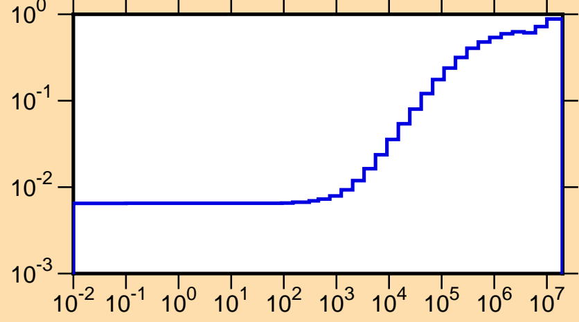
\mu vs. E for ^{111}\text{Cd}(\text{mt251})
