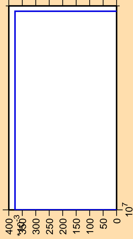
\Delta\sigma/\sigma vs. E for ^{111}\text{Cd}(n,\text{nt})
