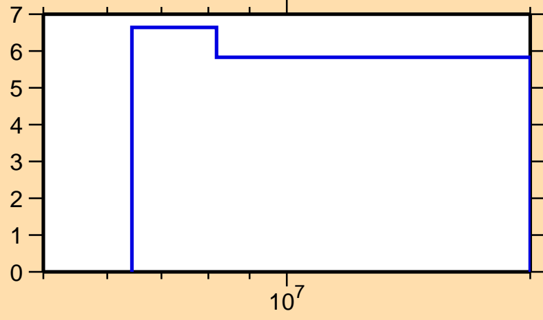
\Delta\sigma/\sigma vs. E for ^{111}\text{Cd}(n,\text{el.})
