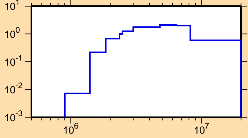
\sigma vs. E for ^{111}\text{Cd}(n,n\text{cont.})
