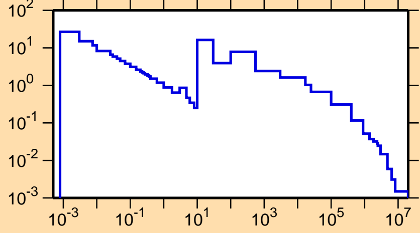
\sigma vs. E for ^{111}\text{Cd}(n,\gamma)
