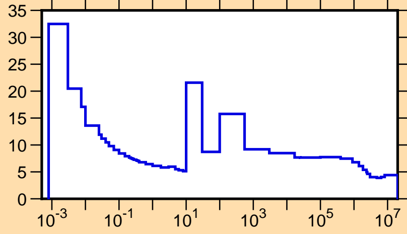
\sigma vs. E for ^{111}\text{Cd}(n,\text{tot.})
