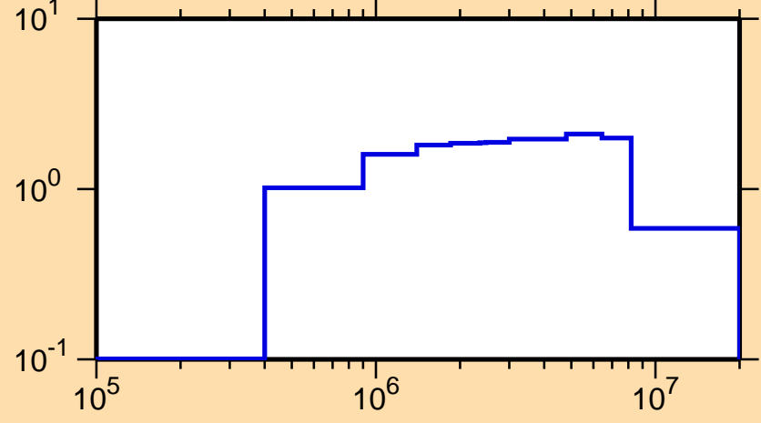
\sigma vs. E for ^{111}\text{Cd}(n,\text{inel.})
