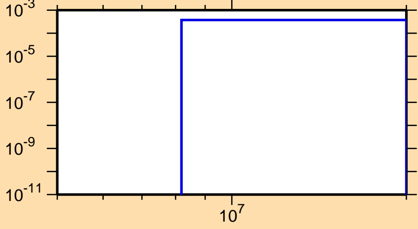
\sigma vs. E for ^{111}\text{Cd}(n,n\alpha)
