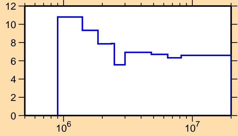
\Delta\sigma/\sigma vs. E for ^{111}\text{Cd}(n,n\text{onel.})
