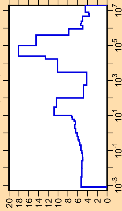
\Delta\sigma/\sigma vs. E for ^{111}\text{Cd}(n,\text{tot.})
