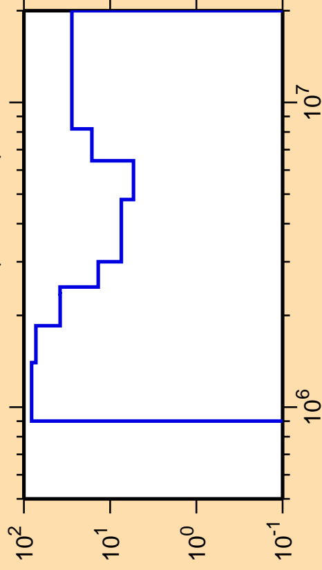
\Delta\sigma/\sigma vs. E for ^{113}\text{Cd}(n,\text{ncont.})
