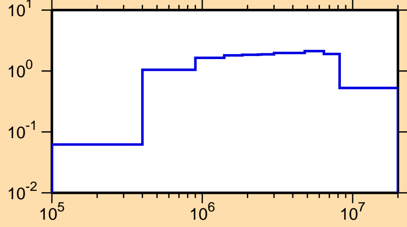
\sigma vs. E for ^{113}\text{Cd}(n,\text{inel.})
