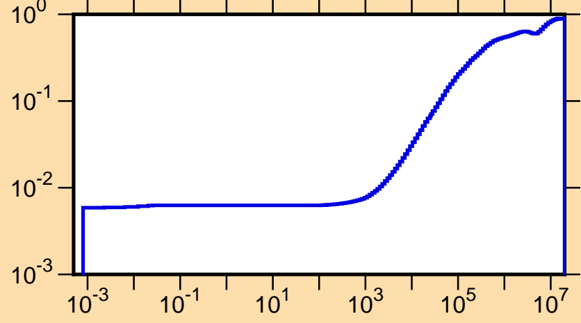
\mu vs. E for ^{115}\text{Cd}(\text{mt251})
