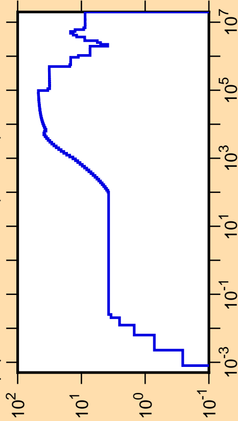
\Delta\mu/\mu vs. E for ^{115}\text{Cd}(\text{mt251})
