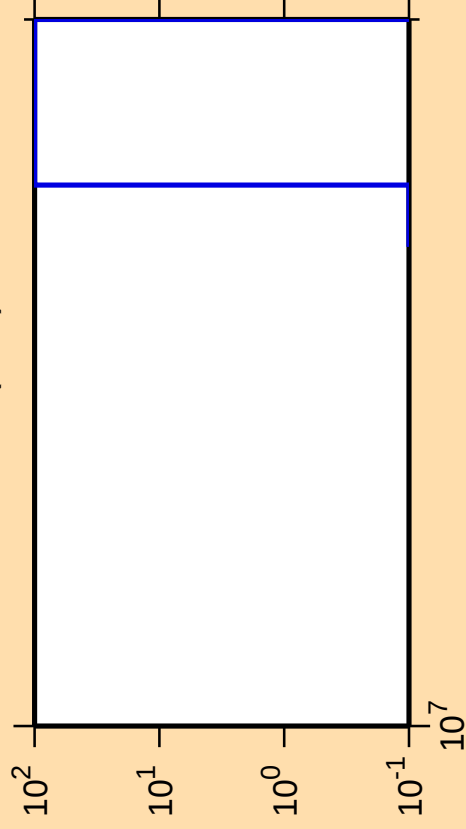
\Delta\sigma/\sigma vs. E for ^{115}\text{Cd}(n,\text{nt})
