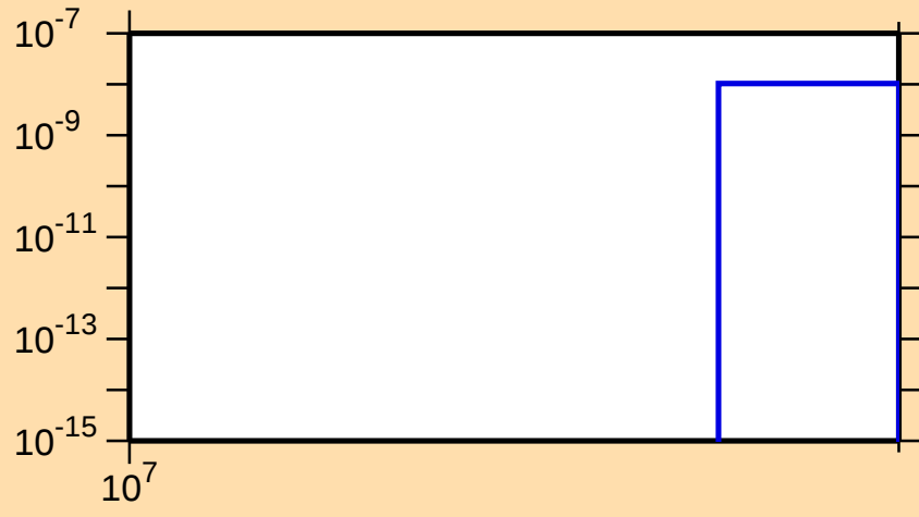
\sigma vs. E for ^{115}\text{Cd}(n,2np)
