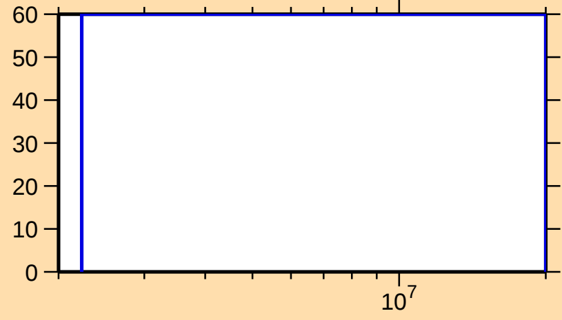
\Delta\sigma/\sigma vs. E for ^{115}\text{Cd}(n,\gamma)
