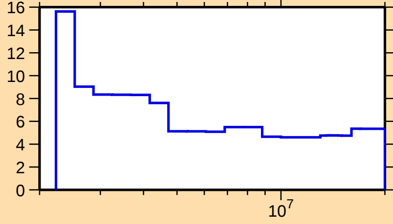
\Delta\sigma/\sigma vs. E for ^{115}\text{Cd}(n,\text{nonel.})
