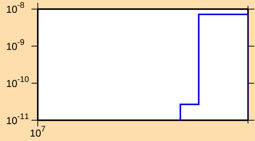
\sigma vs. E for ^{115}\text{Cd}(n,2n\alpha)
