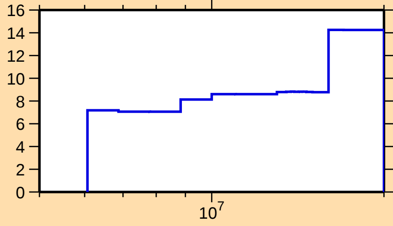
\Delta\sigma/\sigma vs. E for ^{115}\text{Cd}(n,2n)
