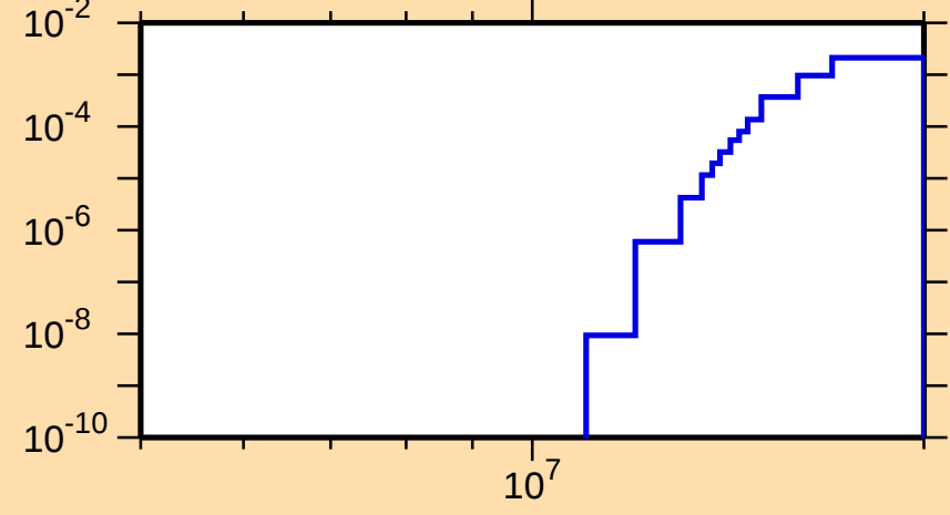
\sigma vs. E for ^{115}\text{Cd}(n,d)
