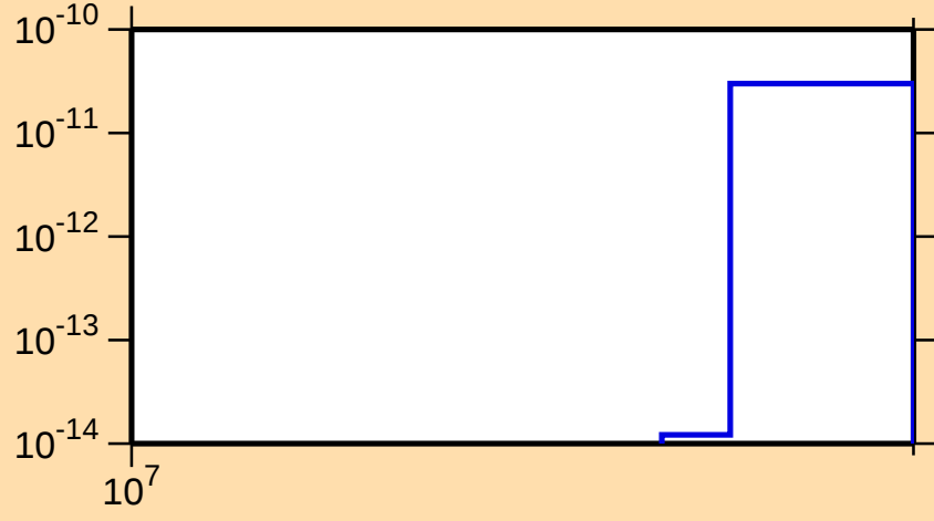
\sigma vs. E for ^{115}\text{Cd}(n,\text{He3})
