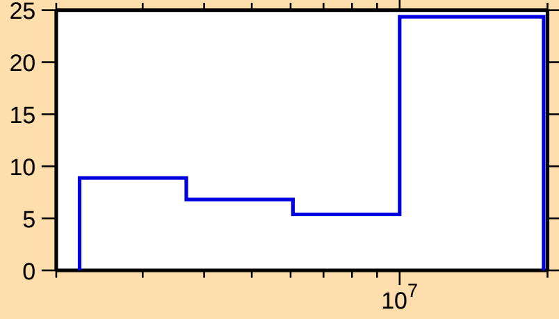
\Delta\sigma/\sigma vs. E for ^{115}\text{Cd}(n,n\text{cont.})
