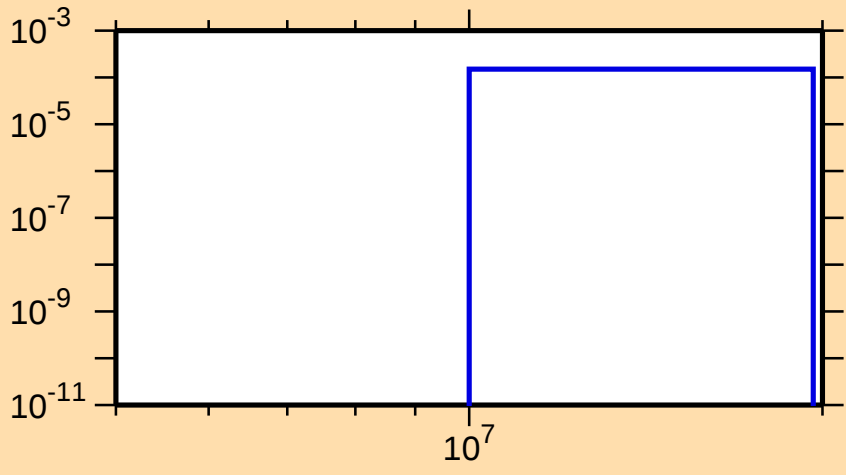
\sigma vs. E for ^{115}\text{Cd}(n,d)
