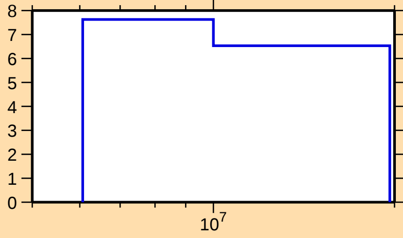
\Delta\sigma/\sigma vs. E for ^{115}\text{Cd}(n,\text{el.})
