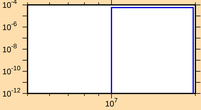
\sigma vs. E for ^{115}\text{Cd}(n,t)
