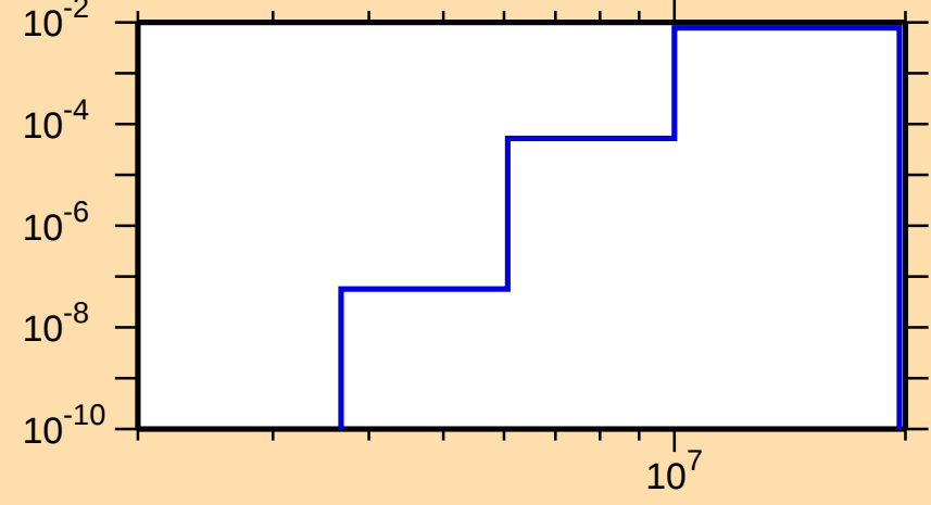
\sigma vs. E for ^{115}\text{Cd}(n,p)
