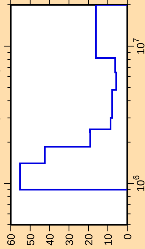
\Delta\sigma/\sigma vs. E for ^{115}\text{Cd}(\text{n},\text{ncont.})
