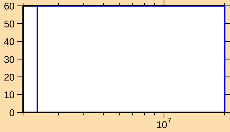
\Delta\sigma/\sigma vs. E for ^{115}\text{Cd}(n,n_1)
