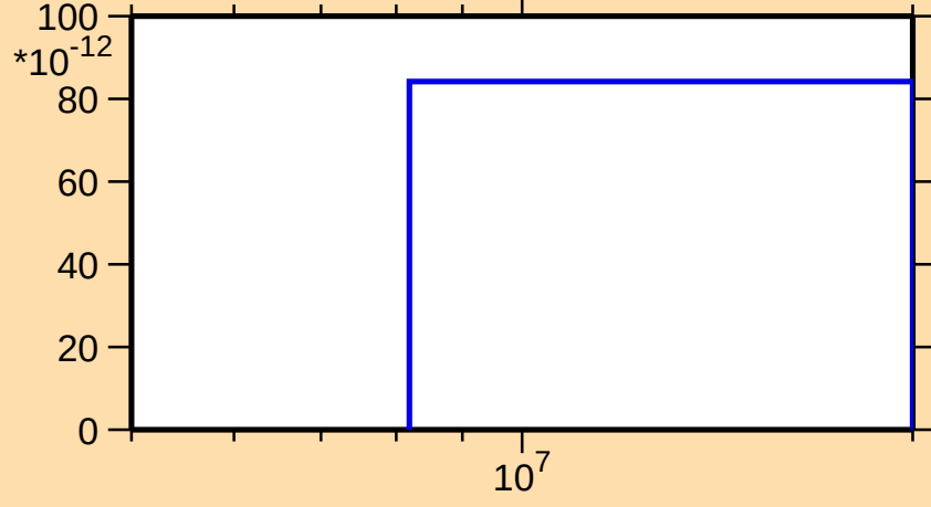
\sigma vs. E for ^{115}\text{Cd}(n,2np)
