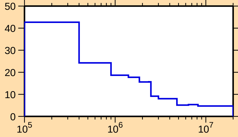
\Delta\sigma/\sigma vs. E for ^{115}\text{Cd}(\text{n,nonel.})
