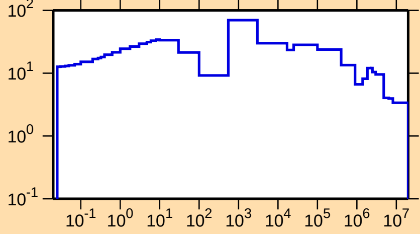
\Delta\sigma/\sigma vs. E for ^{115}\text{Cd}(n,\text{tot.})
