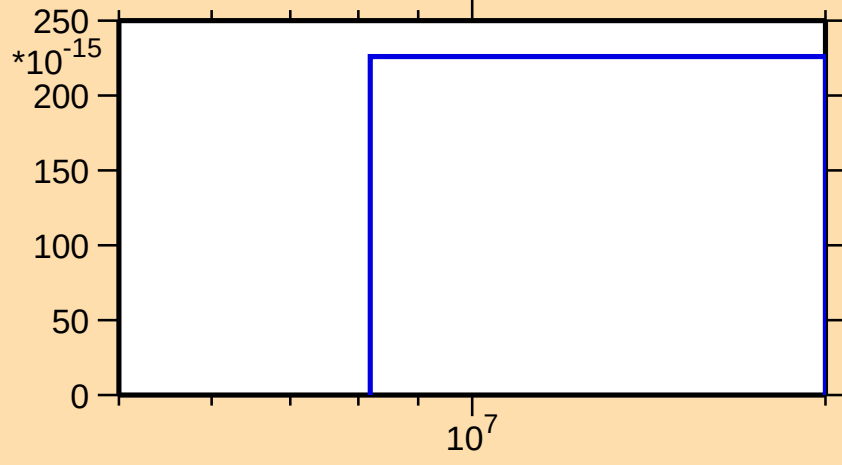
\sigma vs. E for ^{115}\text{Cd}(n,\text{nt})
