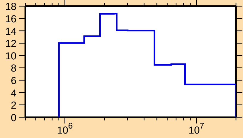
\Delta\sigma/\sigma vs. E for ^{115}\text{Cd}(\text{n},\text{el.})
