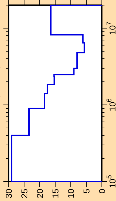
\Delta\sigma/\sigma vs. E for ^{115}\text{Cd}(\text{n,inel.})
