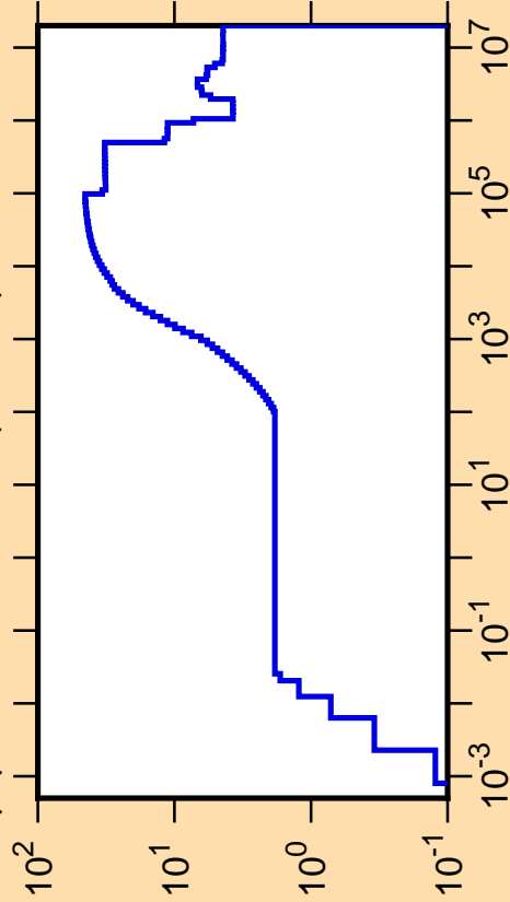
\Delta\mu/\mu vs. E for ^{116}\text{Cd}(\text{mt251})
