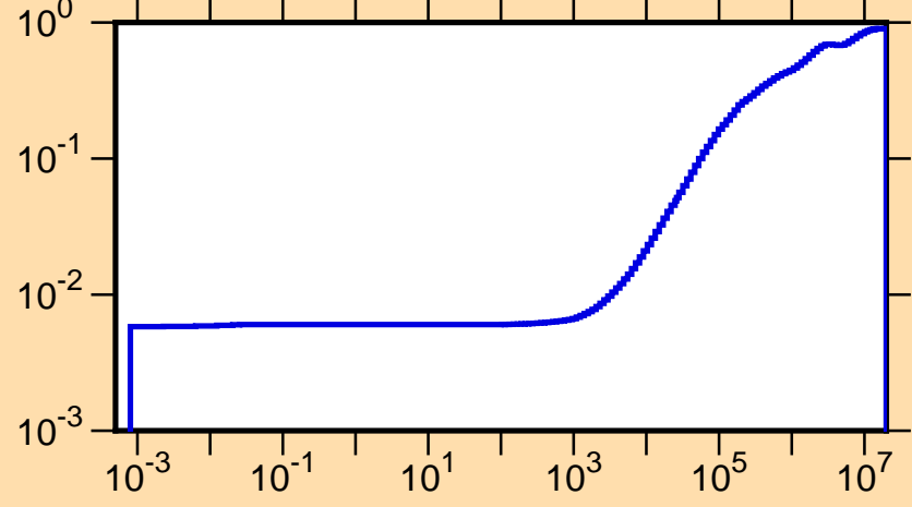
\mu vs. E for ^{116}\text{Cd}(\text{mt251})
