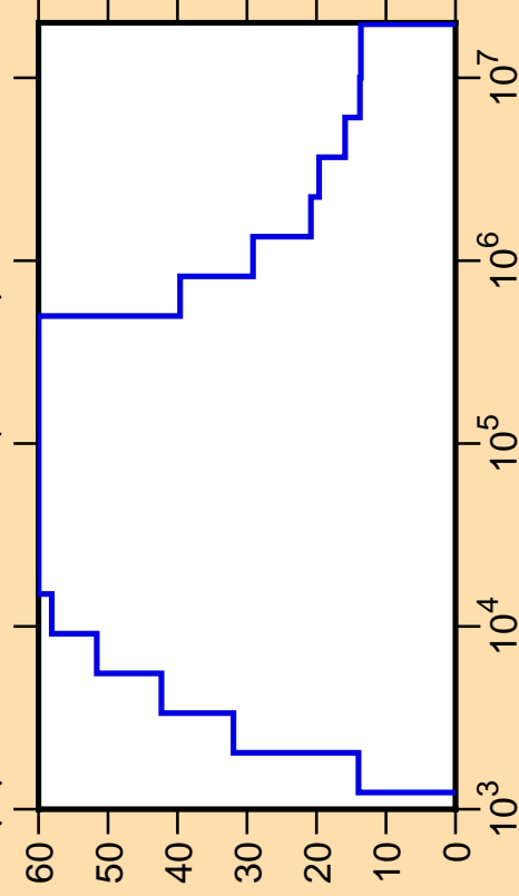
\Delta\mu/\mu vs. E for ^{118}\text{Cd}(\text{mt251})
