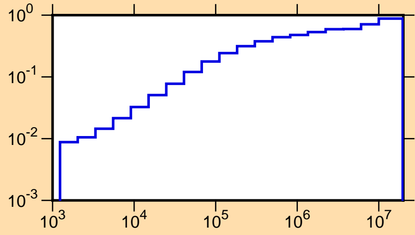
\mu vs. E for ^{118}\text{Cd}(\text{mt251})
