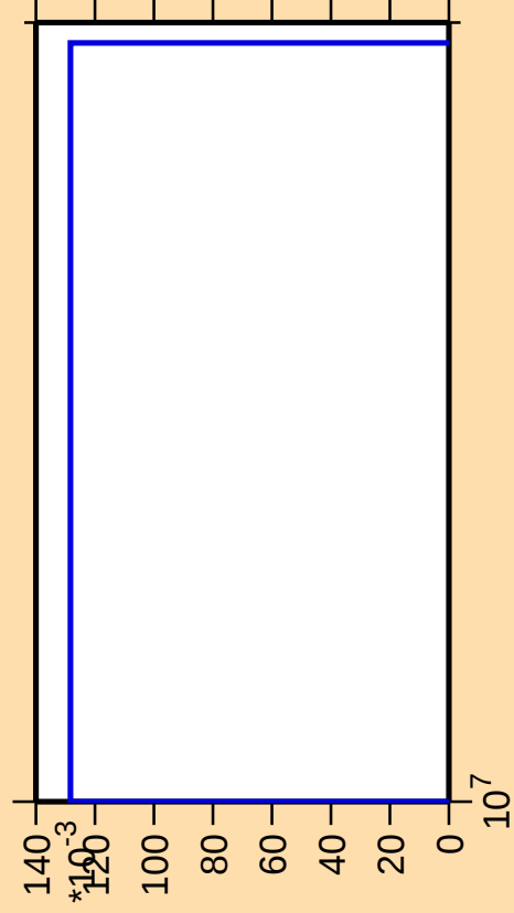
\Delta\sigma/\sigma vs. E for ^{118}\text{Cd}(n,\text{nt})
