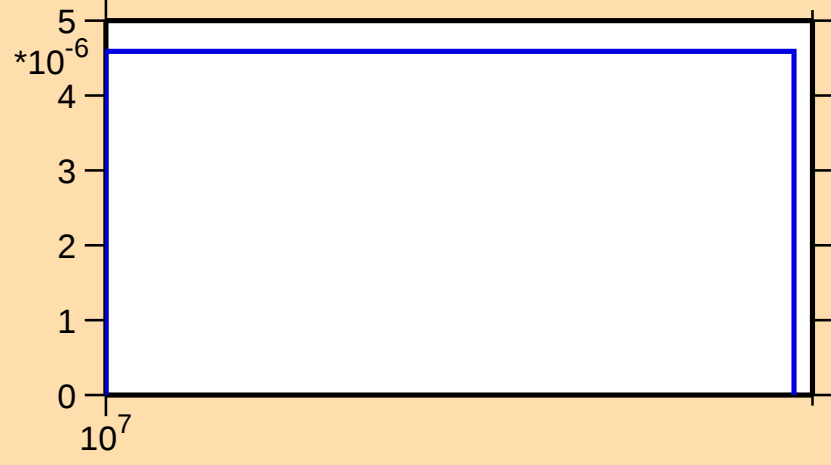
\sigma vs. E for ^{118}\text{Cd}(n,np)
