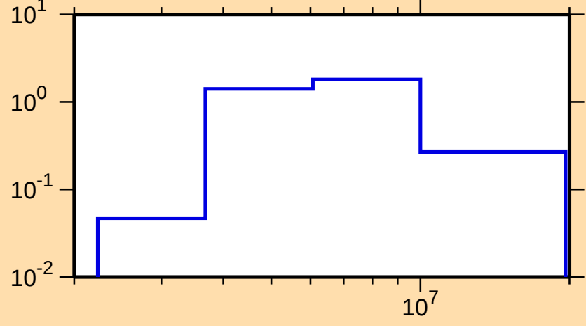
\sigma vs. E for ^{118}\text{Cd}(n,n\text{cont.})
