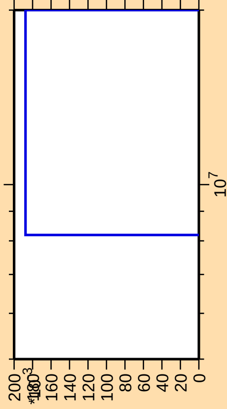
\Delta\sigma/\sigma vs. E for ^{118}\text{Cd}(n,\text{nt})
