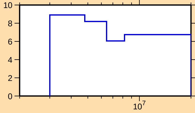
\Delta\sigma/\sigma vs. E for ^{118}\text{Cd}(\text{n},\text{nonel.})
