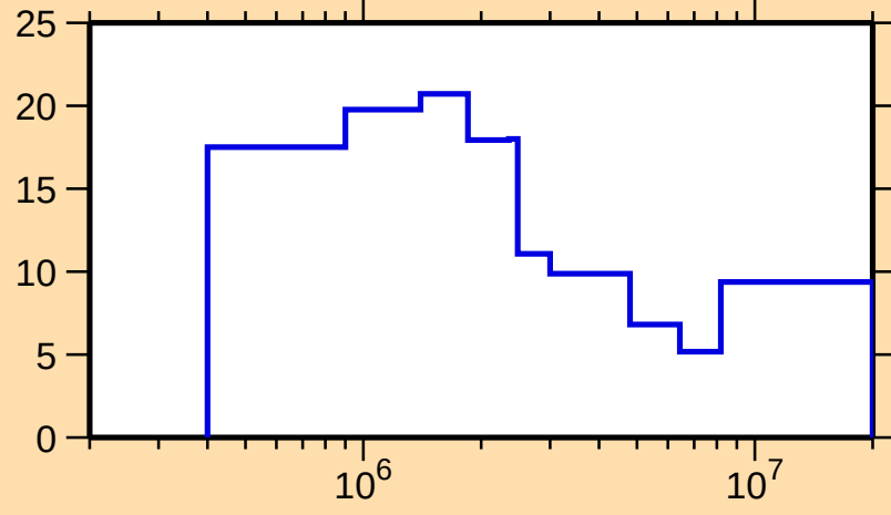
\Delta\sigma/\sigma vs. E for ^{118}\text{Cd}(\text{n,tot.})
