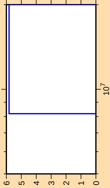
\Delta\sigma/\sigma vs. E for ^{118}\text{Cd}(n,2n)
