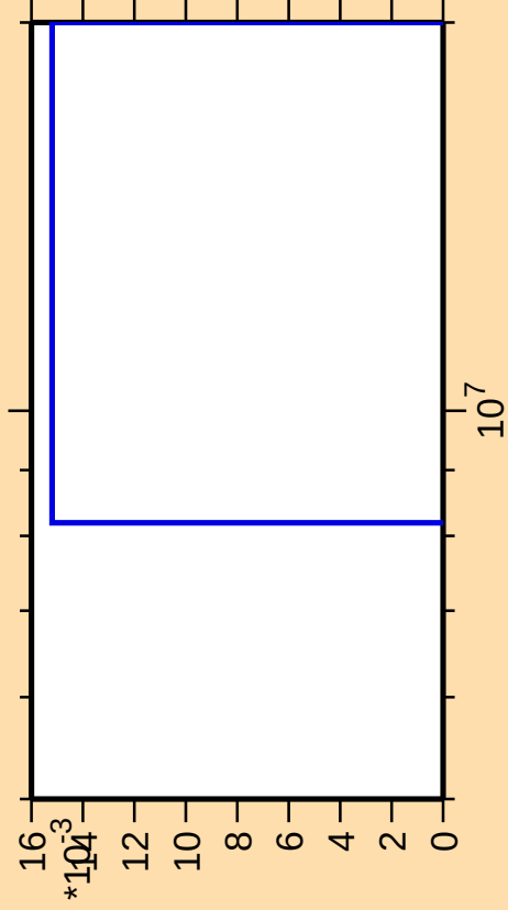
\Delta\sigma/\sigma vs. E for ^{118}\text{Cd}(n,\text{nd})
