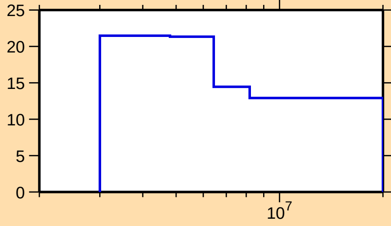
\Delta\sigma/\sigma vs. E for ^{118}\text{Cd}(\text{n},\text{el.})
