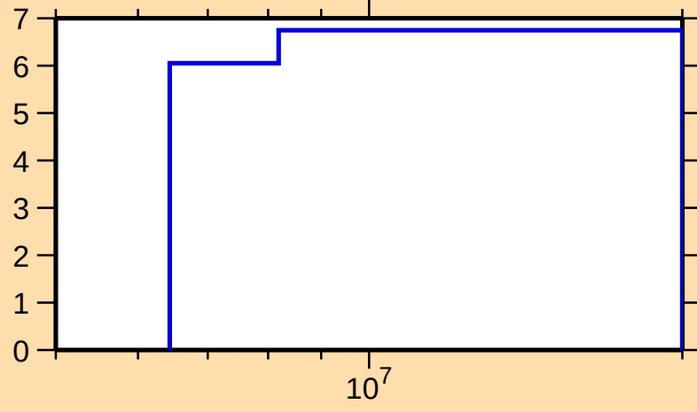
\Delta\sigma/\sigma vs. E for ^{118}\text{Cd}(n,\text{nonel.})
