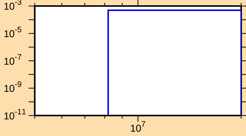
\sigma vs. E for ^{118}\text{Cd}(n,p)
