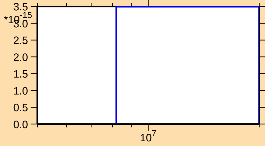
\sigma vs. E for ^{118}\text{Cd}(n,\text{nd})
