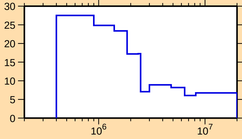
\Delta\sigma/\sigma vs. E for ^{118}\text{Cd}(\text{n,nonel.})
