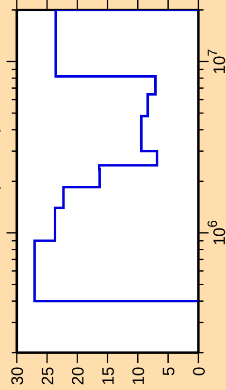
\Delta\sigma/\sigma vs. E for ^{118}\text{Cd}(\text{n,inel.})
