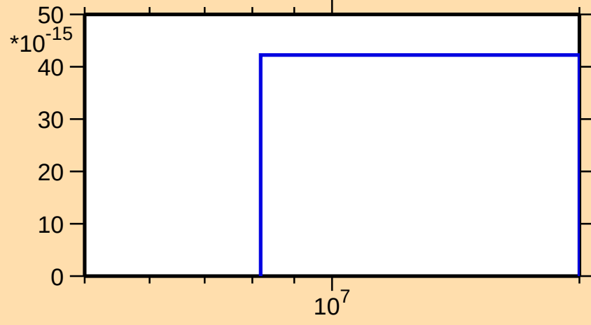
\sigma vs. E for ^{118}\text{Cd}(n,\text{nt})
