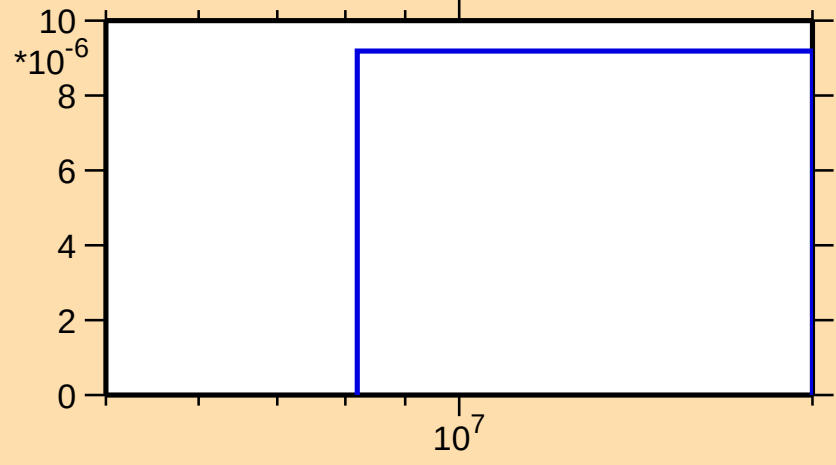
\sigma vs. E for ^{118}\text{Cd}(n,d)
