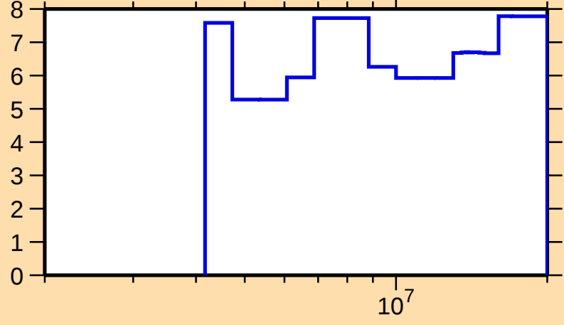
\Delta\sigma/\sigma vs. E for ^{119}\text{Cd}(n,\text{nonel.})
