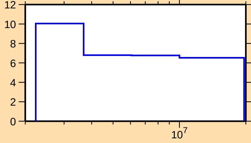
\Delta\sigma/\sigma vs. E for ^{119}\text{Cd}(n,n\text{oncl.})
