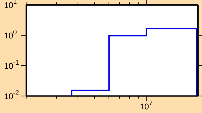
\sigma vs. E for ^{119}\text{Cd}(n,2n)
