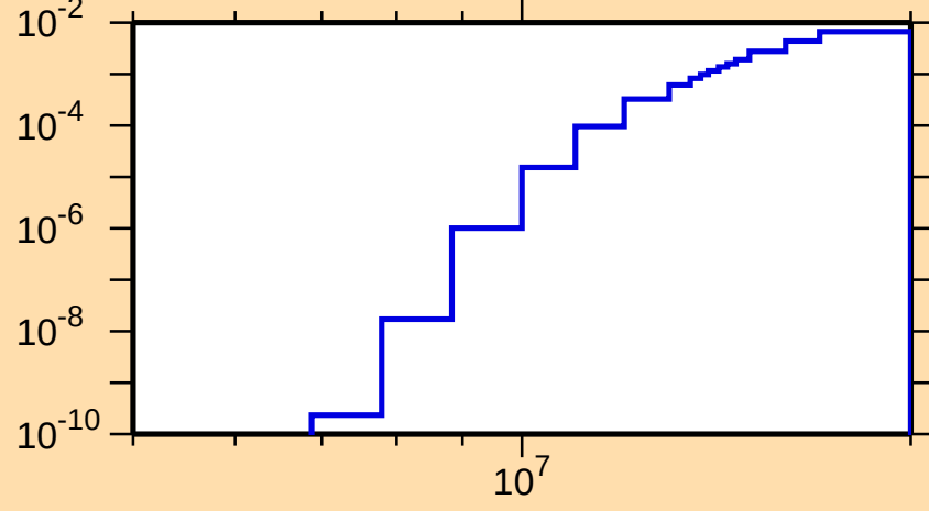
\sigma vs. E for ^{119}\text{Cd}(n,p)
