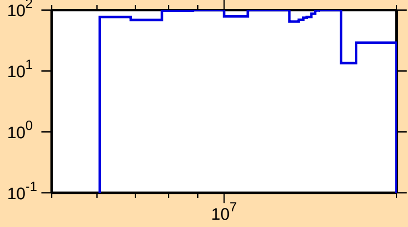
\Delta\sigma/\sigma vs. E for ^{119}\text{Cd}(n,n_1)
