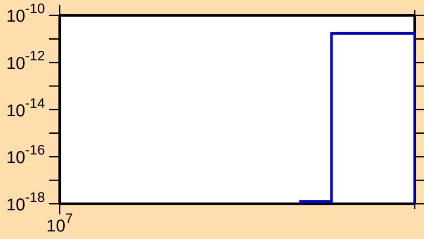
\sigma vs. E for ^{119}\text{Cd}(n,\text{nt})
