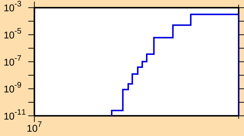
\sigma vs. E for ^{119}\text{Cd}(n,np)
