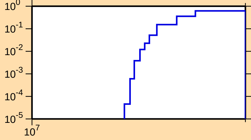
\sigma vs. E for ^{119}\text{Cd}(n,3n)
