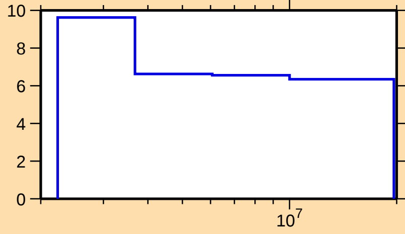
\Delta\sigma/\sigma vs. E for ^{119}\text{Cd}(\text{n},\text{nonel.})
