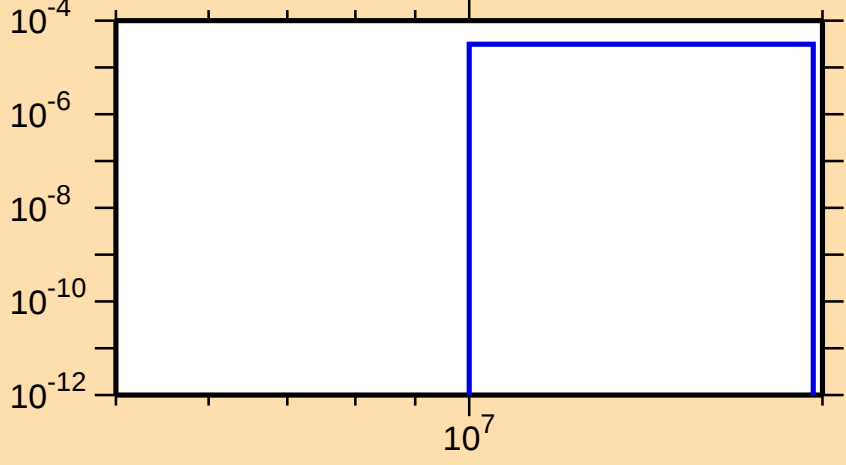
\sigma vs. E for ^{119}\text{Cd}(n,d)
