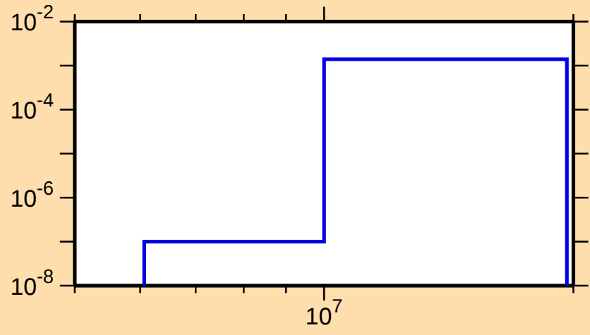
\sigma vs. E for ^{119}\text{Cd}(n,p)
