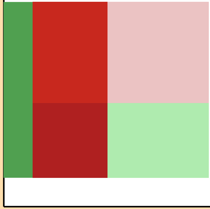
\Delta\sigma/\sigma vs. E for ^{119}\text{Cd}(n,\text{tot.})
