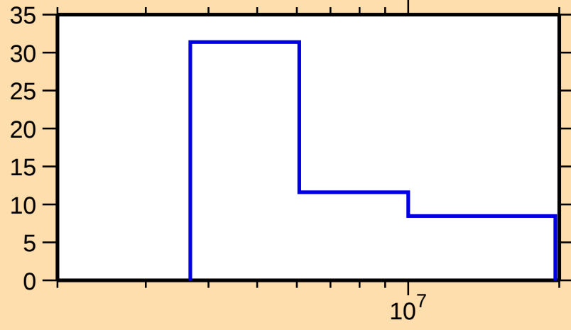
\Delta\sigma/\sigma vs. E for ^{119}\text{Cd}(n,2n)
