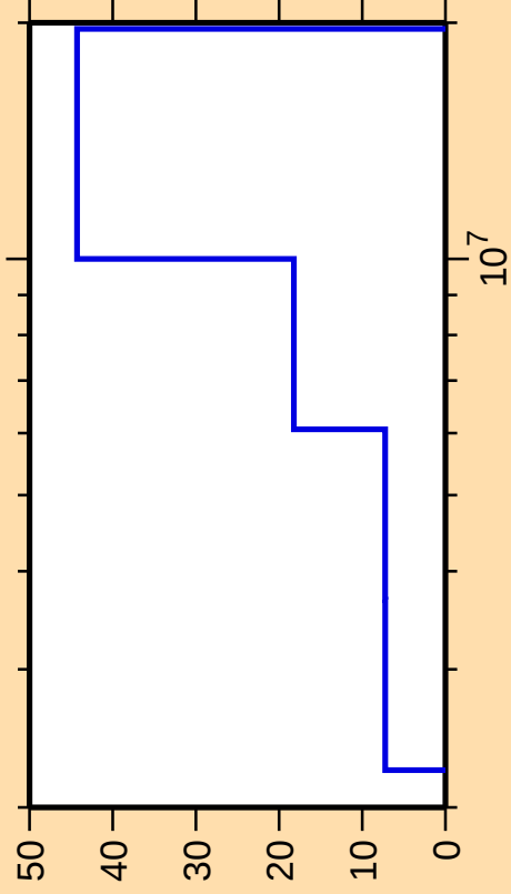
\Delta\sigma/\sigma vs. E for ^{119}\text{Cd}(n,\text{ncont.})
