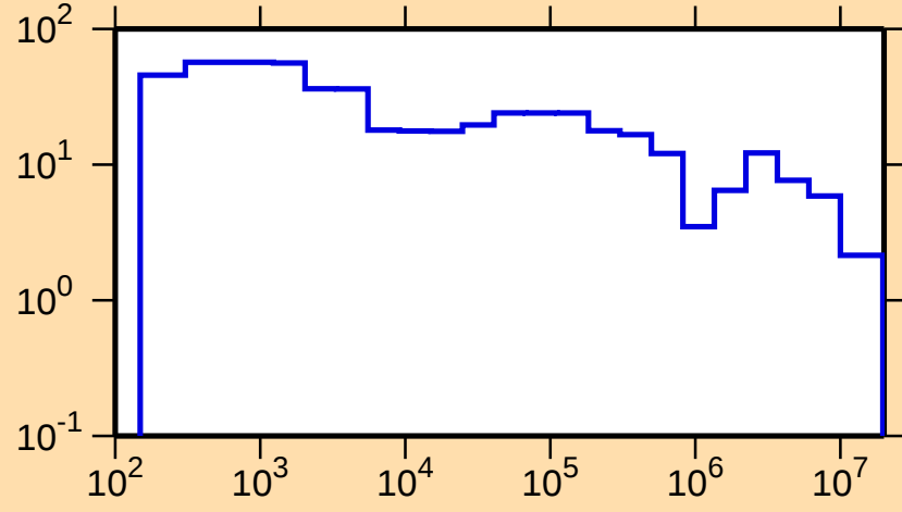
\Delta\sigma/\sigma vs. E for ^{119}\text{Cd}(\text{n,el.})
