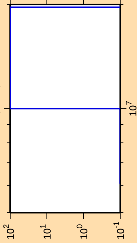
\Delta\sigma/\sigma vs. E for ^{119}\text{Cd}(n,\alpha)
