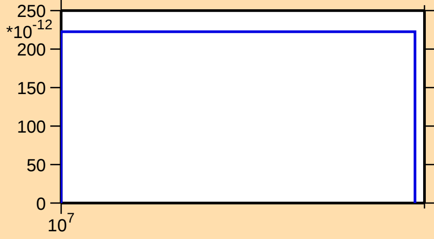
\sigma vs. E for ^{119}\text{Cd}(n,\text{nd})
