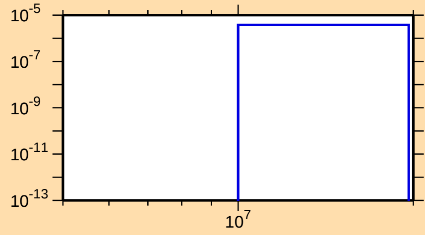
\sigma vs. E for ^{119}\text{Cd}(n,t)
