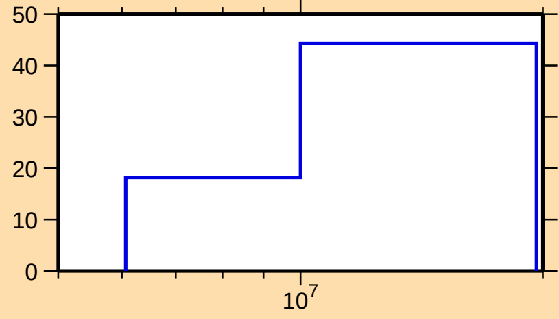
\Delta\sigma/\sigma vs. E for ^{119}\text{Cd}(n,n\text{cont.})
