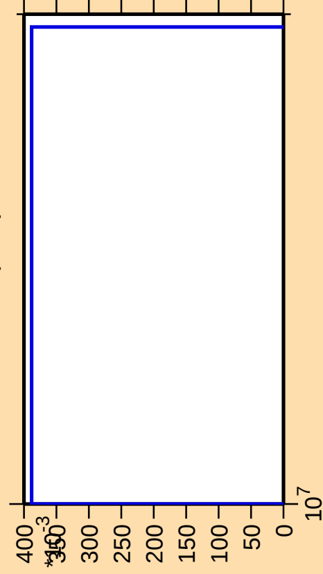
\Delta\sigma/\sigma vs. E for ^{119}\text{Cd}(n,\text{nt})
