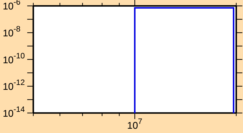
\sigma vs. E for ^{119}\text{Cd}(n,\alpha)
