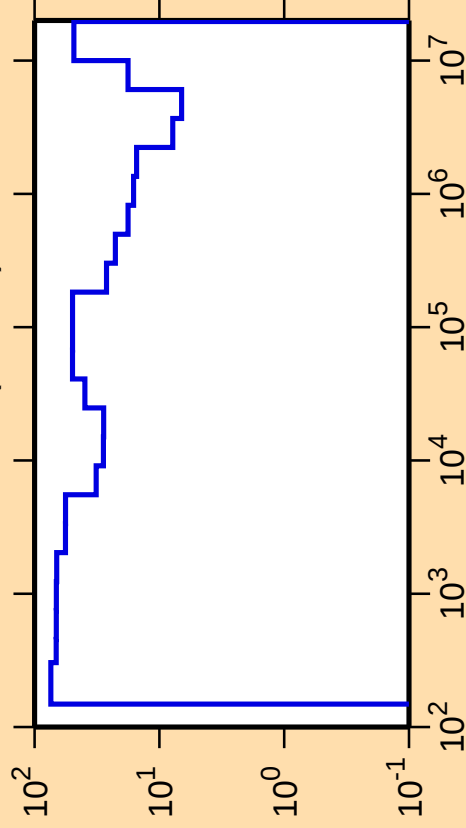
\Delta\sigma/\sigma vs. E for ^{119}\text{Cd}(\text{n,inel.})
