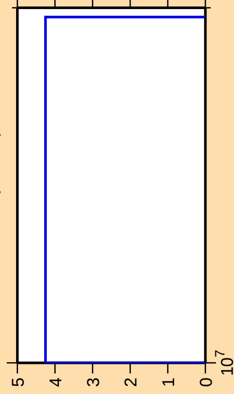
\Delta\sigma/\sigma vs. E for ^{119}\text{Cd}(n,2n\alpha)
