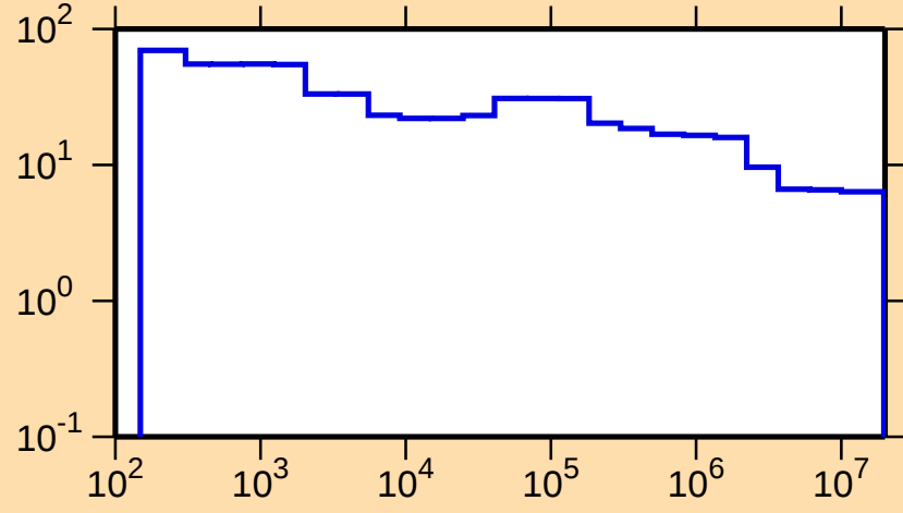
\Delta\sigma/\sigma vs. E for ^{119}\text{Cd}(\text{n,nonel.})
