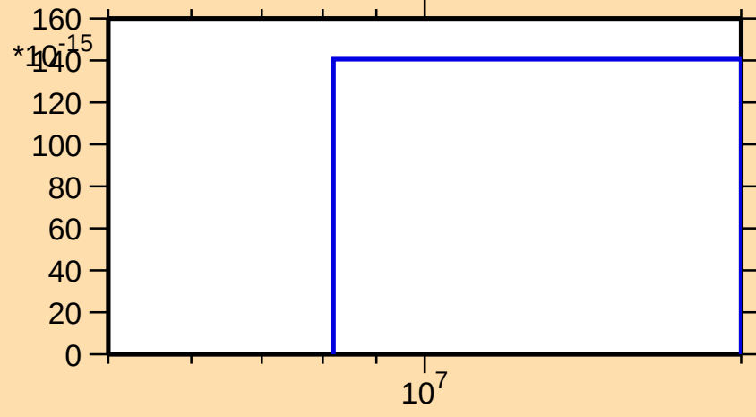
\sigma vs. E for ^{119}\text{Cd}(n,\text{nt})
