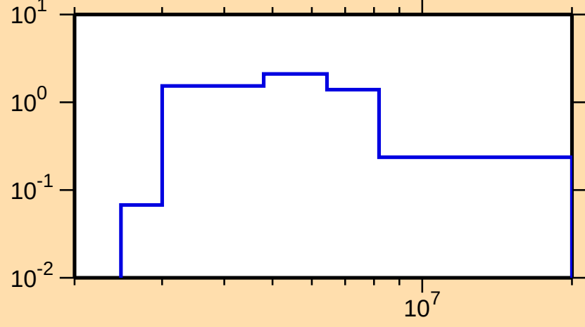
\sigma vs. E for ^{119}\text{Cd}(n,n\text{cont.})
