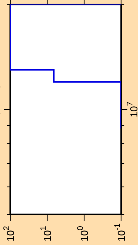
\Delta\sigma/\sigma vs. E for ^{120}\text{Cd}(n,\alpha)
