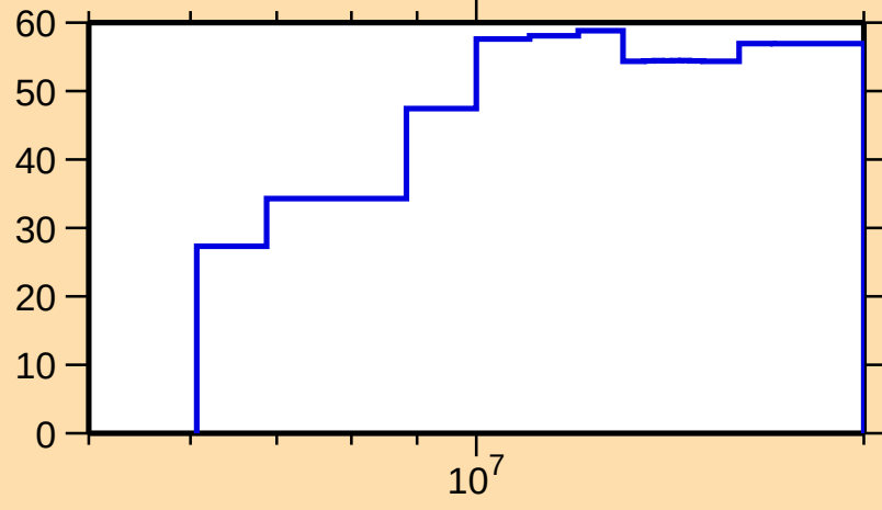
\Delta\sigma/\sigma vs. E for ^{120}\text{Cd}(n,n\text{cont.})
