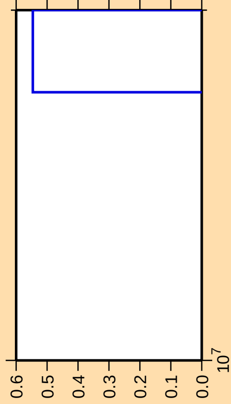
\Delta\sigma/\sigma vs. E for ^{120}\text{Cd}(n,\text{nd})
