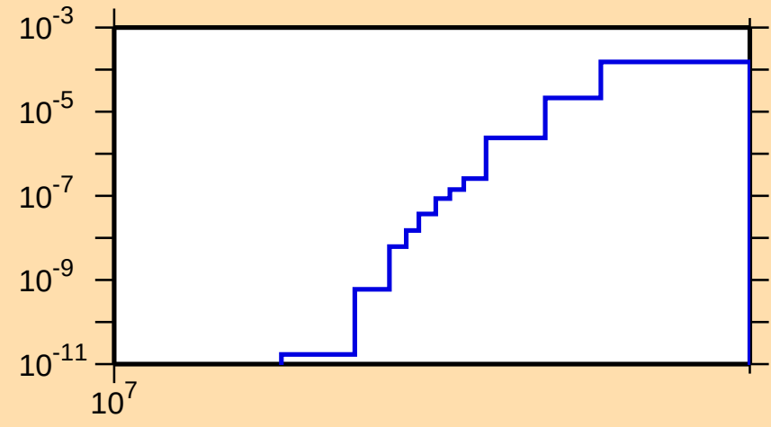
\sigma vs. E for ^{120}\text{Cd}(n,d)
