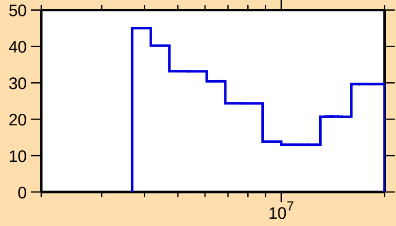
\Delta\sigma/\sigma vs. E for ^{120}\text{Cd}(\text{n},\text{el.})
