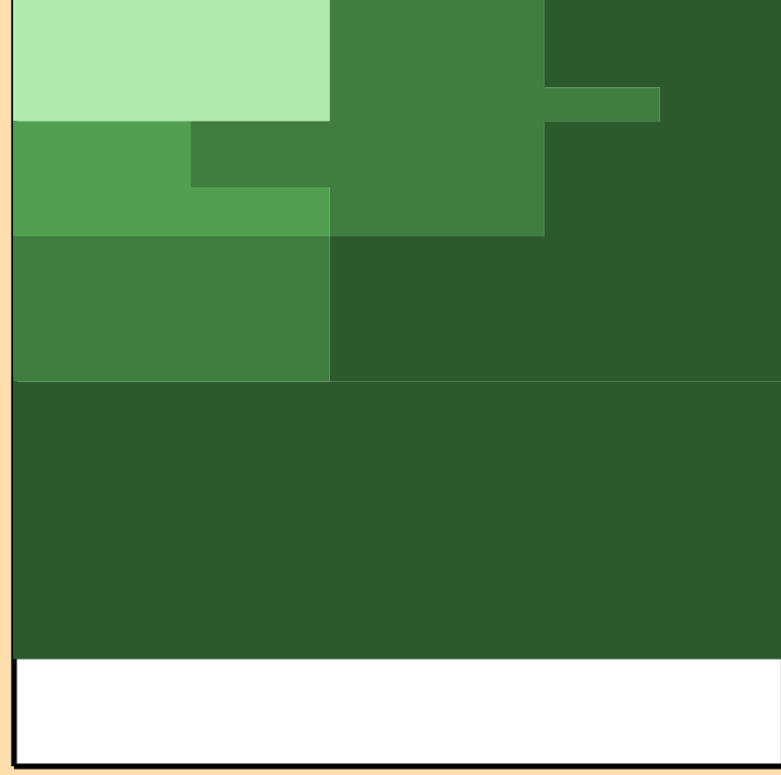
\Delta\sigma/\sigma vs. E for ^{120}\text{Cd}(n,\text{tot.})
