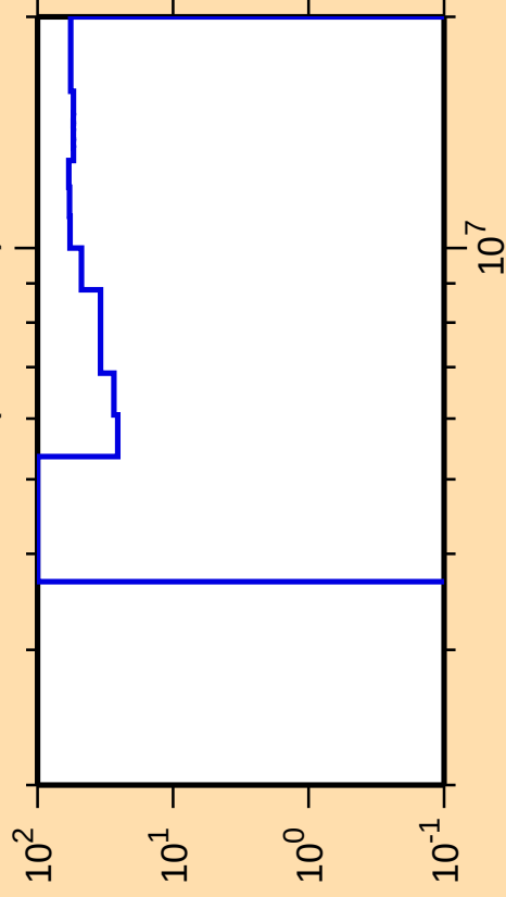
\Delta\sigma/\sigma vs. E for ^{120}\text{Cd}(\text{n},\text{ncont.})
