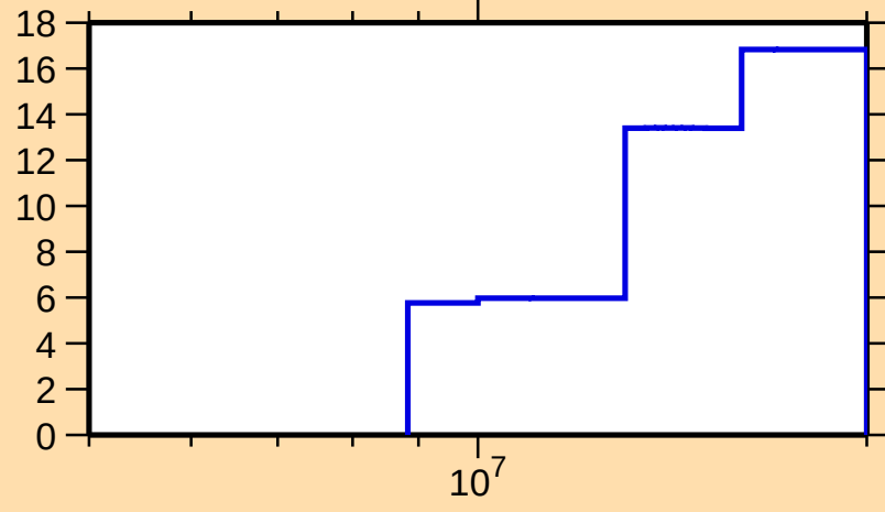
\Delta\sigma/\sigma vs. E for ^{120}\text{Cd}(n,\text{tot.})
