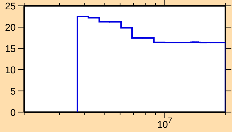
\Delta\sigma/\sigma vs. E for ^{120}\text{Cd}(\text{n},\text{nonel.})
