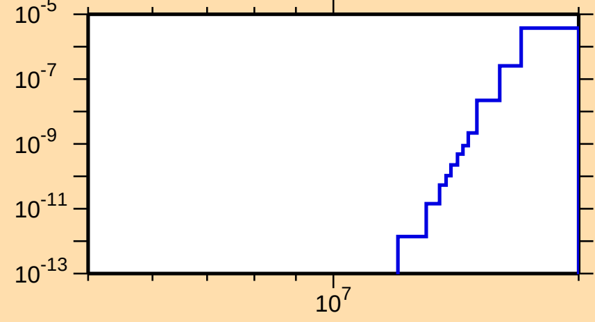
\sigma vs. E for ^{120}\text{Cd}(n,\alpha)
