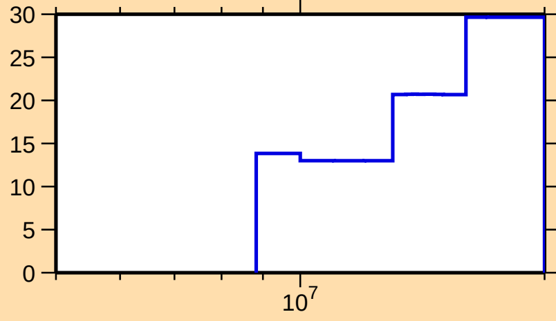
\Delta\sigma/\sigma vs. E for ^{120}\text{Cd}(n,\text{el.})
