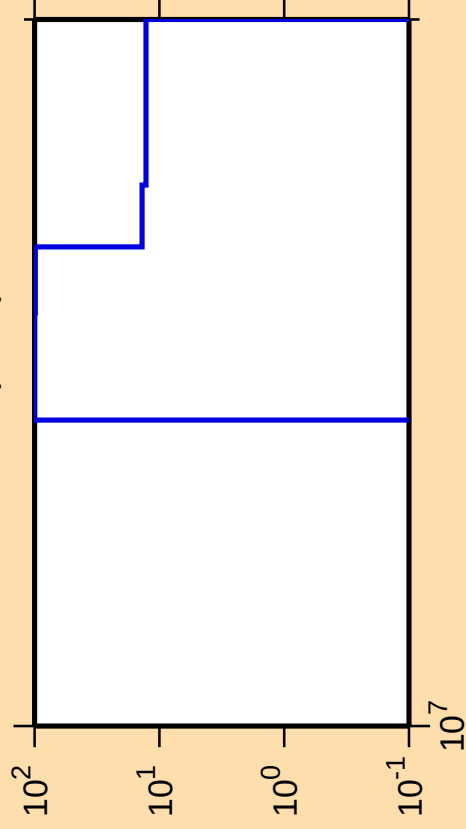
\Delta\sigma/\sigma vs. E for ^{120}\text{Cd}(n,3n)
