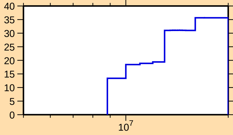
\Delta\sigma/\sigma vs. E for ^{120}\text{Cd}(n,\text{inel.})
