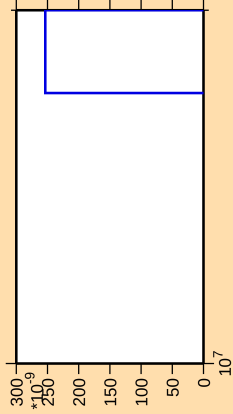
\Delta\sigma/\sigma vs. E for ^{120}\text{Cd}(n,2np)
