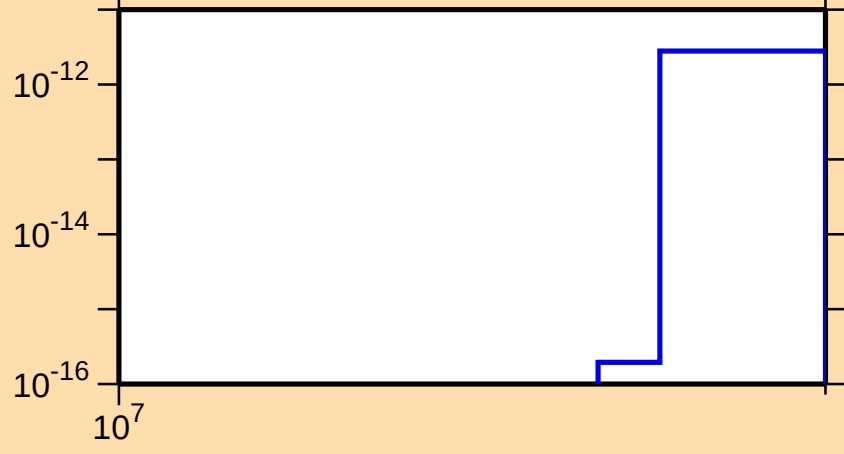
\sigma vs. E for ^{120}\text{Cd}(n,nt)
