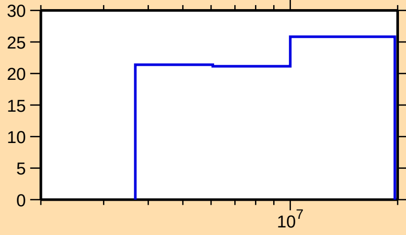
\Delta\sigma/\sigma vs. E for ^{120}\text{Cd}(\text{n,inel.})
