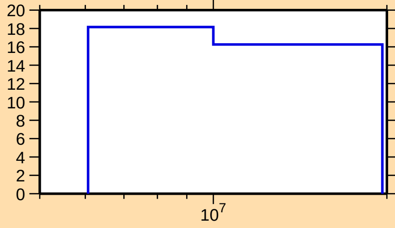
\Delta\sigma/\sigma vs. E for ^{120}\text{Cd}(n,\text{nonel.})
