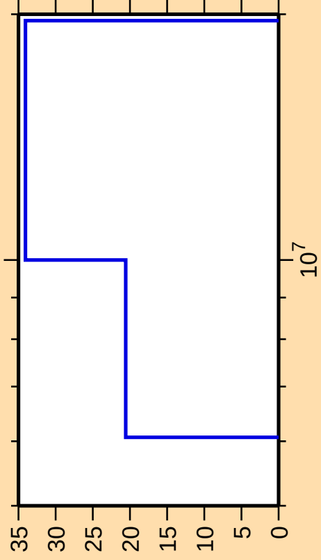
\Delta\sigma/\sigma vs. E for ^{120}\text{Cd}(n,2n)
