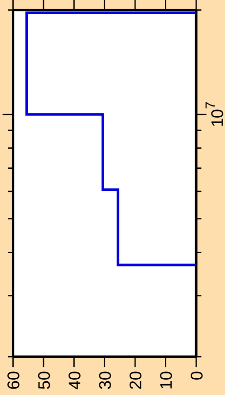
\Delta\sigma/\sigma vs. E for ^{120}\text{Cd}(\text{n,ncont.})
