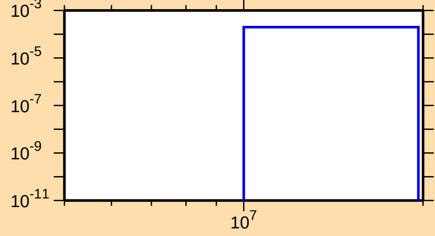
\sigma vs. E for ^{120}\text{Cd}(n,p)
