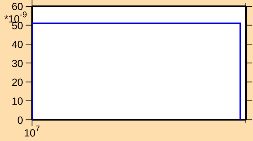
\sigma vs. E for ^{120}\text{Cd}(n,n\alpha)
