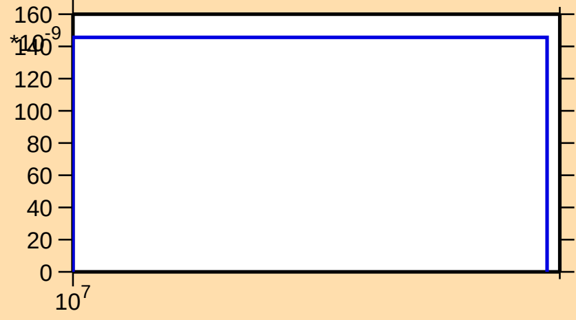
\sigma vs. E for ^{120}\text{Cd}(n,t)
