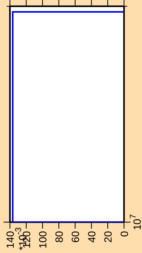
\Delta\sigma/\sigma vs. E for ^{120}\text{Cd}(n,\text{nt})
