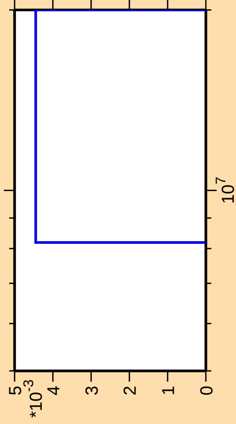
\Delta\sigma/\sigma vs. E for ^{120}\text{Cd}(n,\text{nd})
