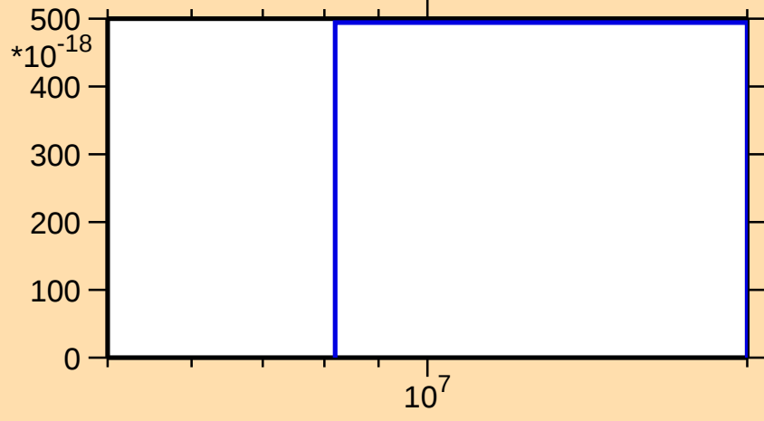
\sigma vs. E for ^{120}\text{Cd}(n,\text{nd})
