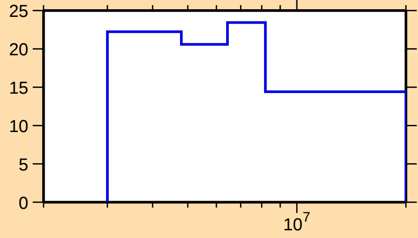
\Delta\sigma/\sigma vs. E for ^{120}\text{Cd}(\text{n},\text{inel.})
