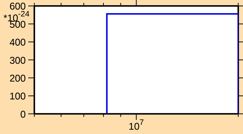
\sigma vs. E for ^{120}\text{Cd}(n,2np)
