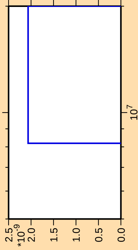
\Delta\sigma/\sigma vs. E for ^{120}\text{Cd}(n,2np)
