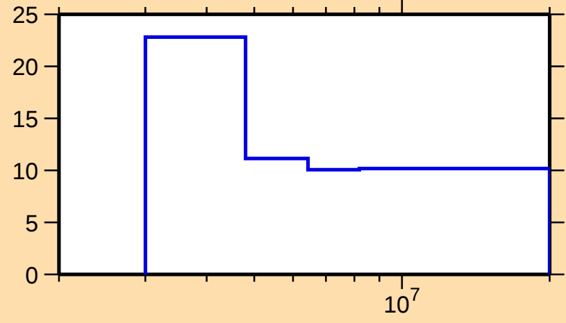
\Delta\sigma/\sigma vs. E for ^{120}\text{Cd}(\text{n,tot.})
