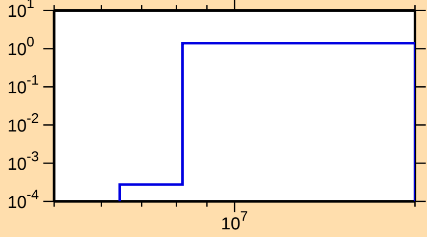
\sigma vs. E for ^{120}\text{Cd}(n,2n)
