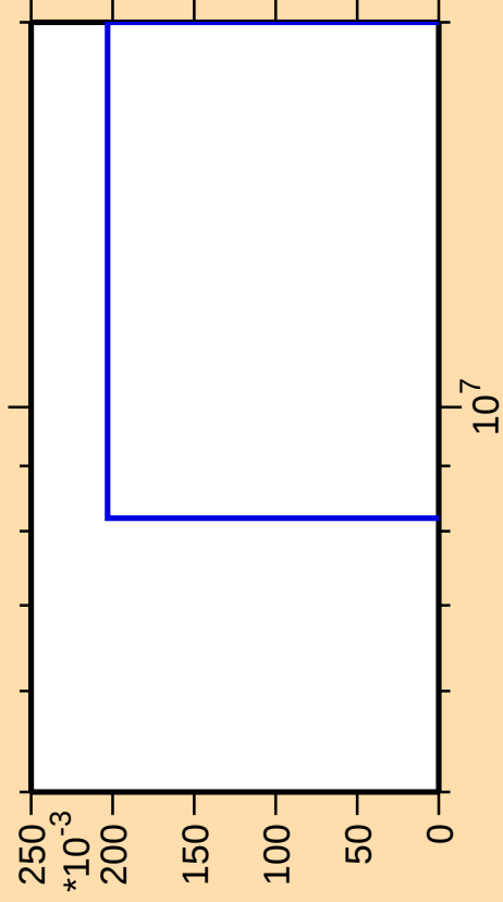
\Delta\sigma/\sigma vs. E for ^{120}\text{Cd}(n,\text{nt})
