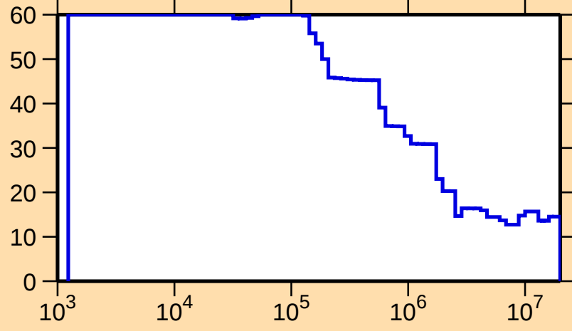
\Delta\sigma/\sigma vs. E for ^{121}\text{Cd}(\text{n,nonel.})
