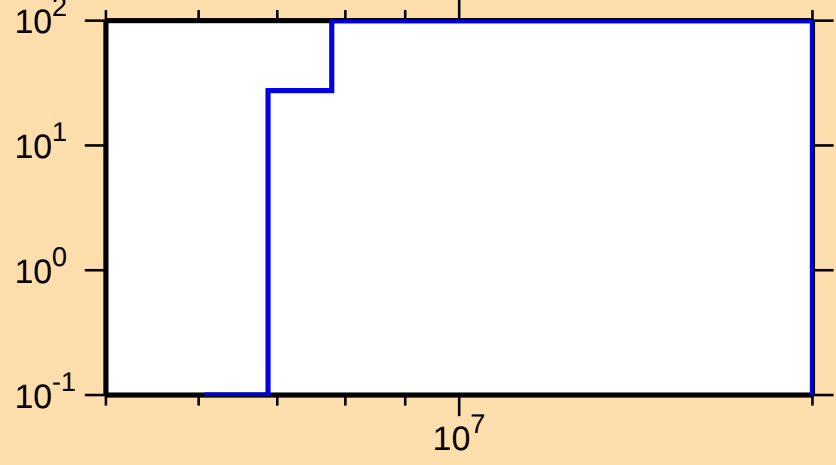
\Delta\sigma/\sigma vs. E for ^{121}\text{Cd}(n,p)
