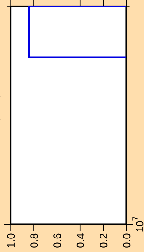
\Delta\sigma/\sigma vs. E for ^{122}\text{Cd}(n,nt)
