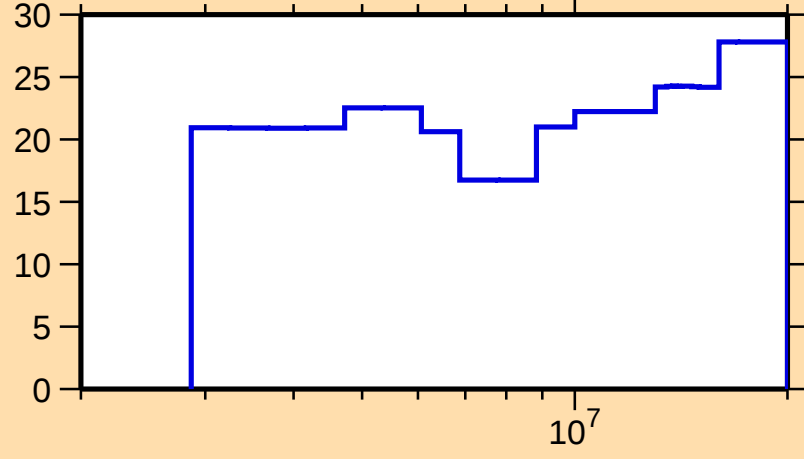
\Delta\sigma/\sigma vs. E for ^{122}\text{Cd}(\text{n},\text{nonel.})
