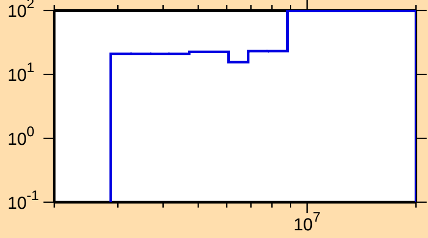
\Delta\sigma/\sigma vs. E for ^{122}\text{Cd}(n,\text{inel.})
