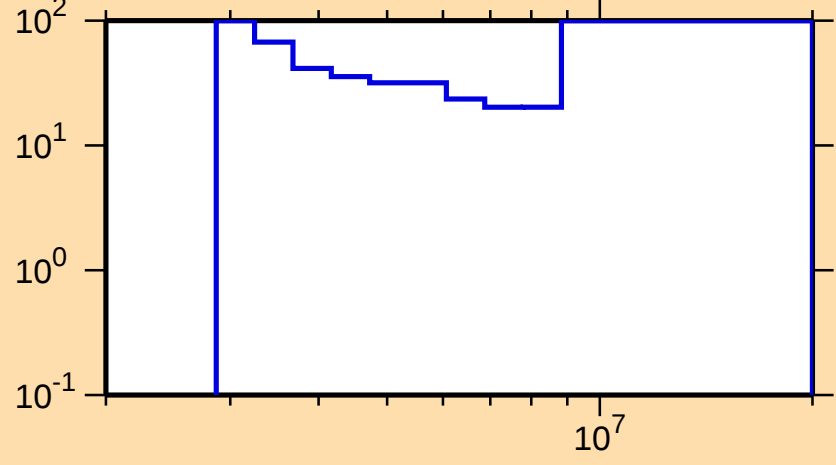
\Delta\sigma/\sigma vs. E for ^{122}\text{Cd}(n,n\text{cont.})
