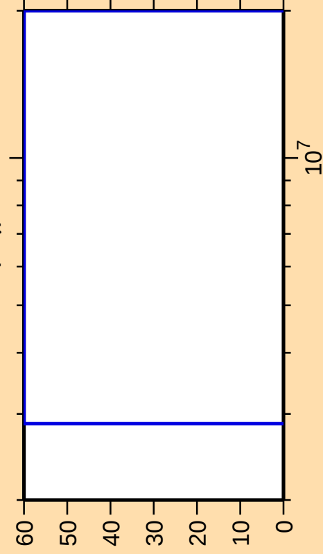
\Delta\sigma/\sigma vs. E for ^{122}\text{Cd}(n,\gamma)
