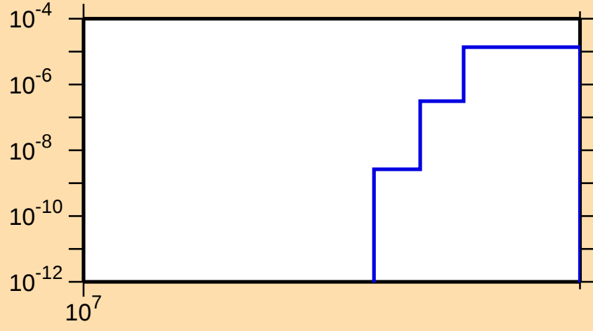
\sigma vs. E for ^{122}\text{Cd}(n,np)
