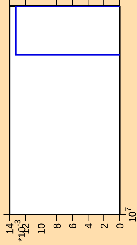
\Delta\sigma/\sigma vs. E for ^{122}\text{Cd}(n,\text{nd})
