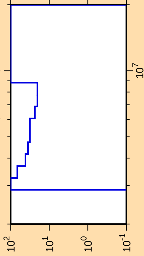
\Delta\sigma/\sigma vs. E for ^{122}\text{Cd}(n,\text{ncont.})
