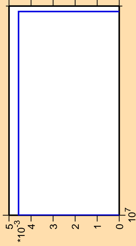
\Delta\sigma/\sigma vs. E for ^{122}\text{Cd}(n,\text{nt})
