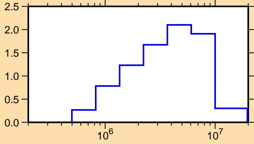
\sigma vs. E for ^{122}\text{Cd}(n,\text{inel.})
