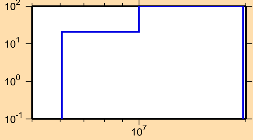
\Delta\sigma/\sigma vs. E for ^{122}\text{Cd}(n,ncont.)
