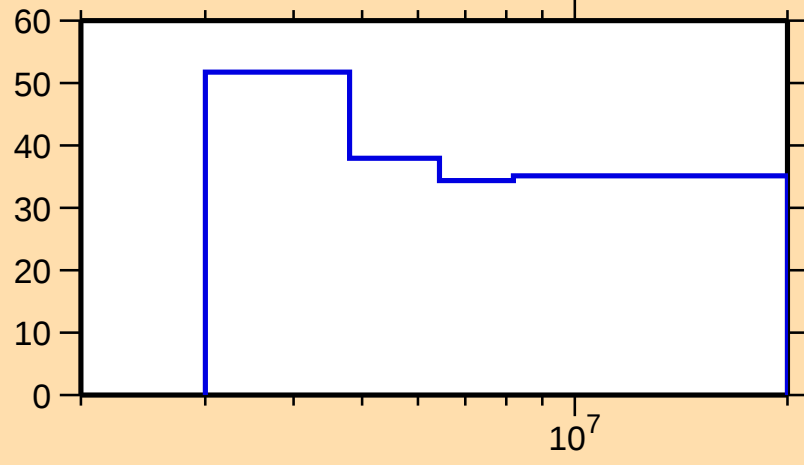
\Delta\sigma/\sigma vs. E for ^{122}\text{Cd}(\text{n},\text{el.})
