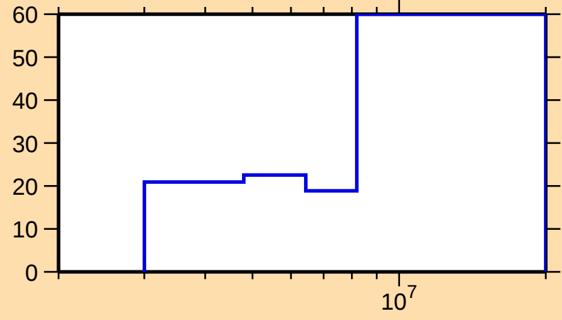
\Delta\sigma/\sigma vs. E for ^{122}\text{Cd}(\text{n},\text{inel.})
