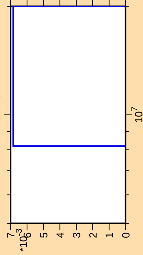
\Delta\sigma/\sigma vs. E for ^{122}\text{Cd}(n,\text{nt})
