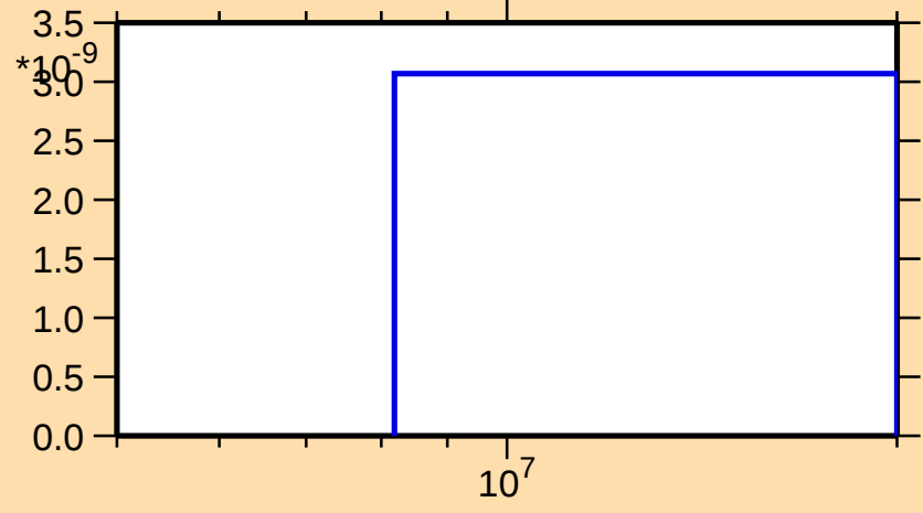
\sigma vs. E for ^{122}\text{Cd}(n,\alpha)
