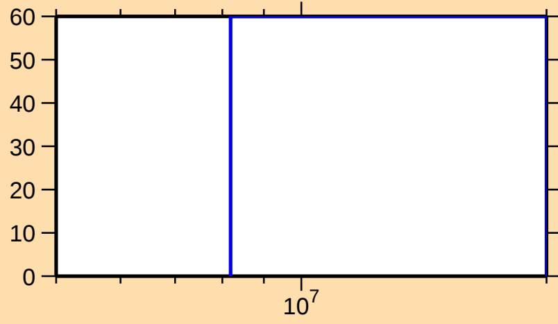
\Delta\sigma/\sigma vs. E for ^{122}\text{Cd}(n,\text{ncont.})
