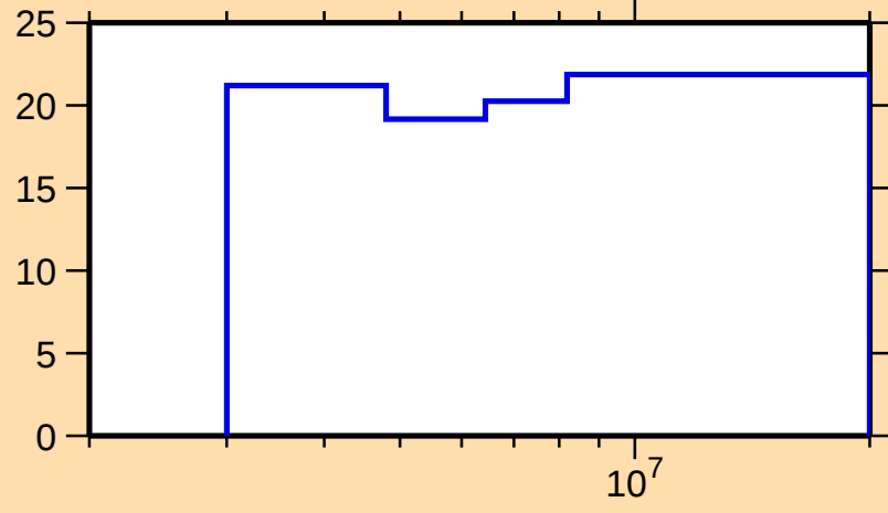
\Delta\sigma/\sigma vs. E for ^{122}\text{Cd}(\text{n},\text{tot.})
